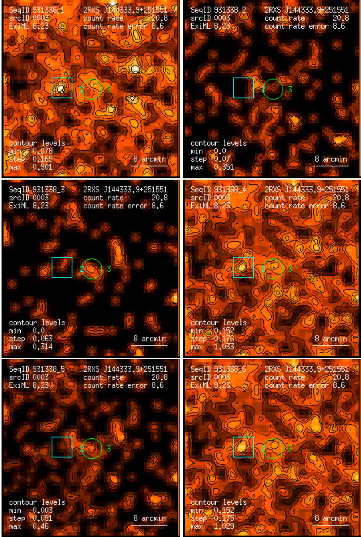
Figure 3: RASS 931338: detection 0003: band rate images, Gaussian filter: (1) PSPC channels 11 – 41, (2) 52 – 90, (3) 91 – 201, (4) 11 – 235, (5) 52 – 201, (6) 11 – 201. Broad band rates in counts/ks. Band rate contour levels in counts/ks/arcmin 2 .
