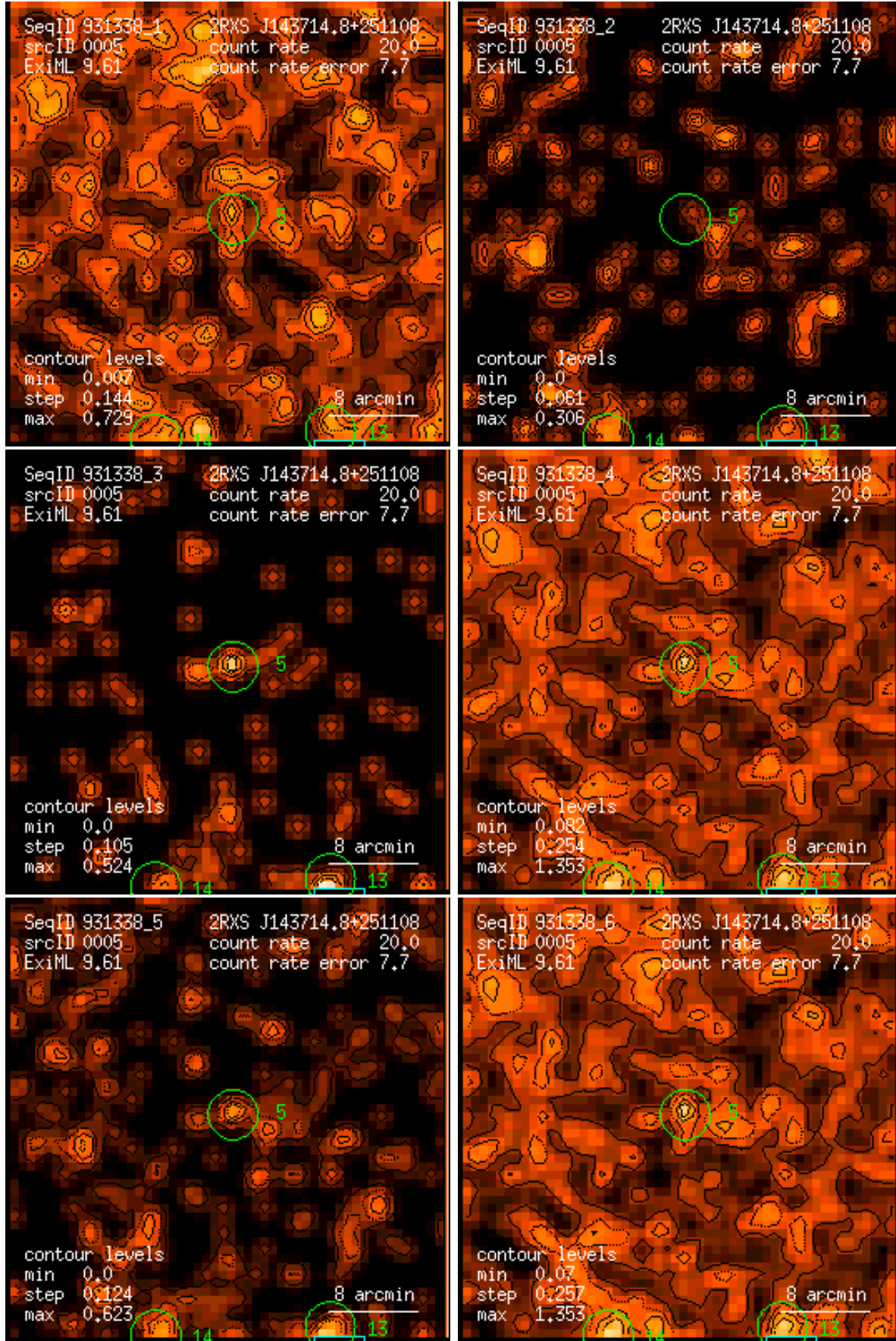
Figure 5: RASS 931338: detection 0005: band rate images, Gaussian filter: (1) PSPC channels 11 – 41, (2) 52 – 90, (3) 91 – 201, (4) 11 – 235, (5) 52 – 201, (6) 11 – 201. Broad band rates in counts/ks. Band rate contour levels in counts/ks/arcmin 2 .
