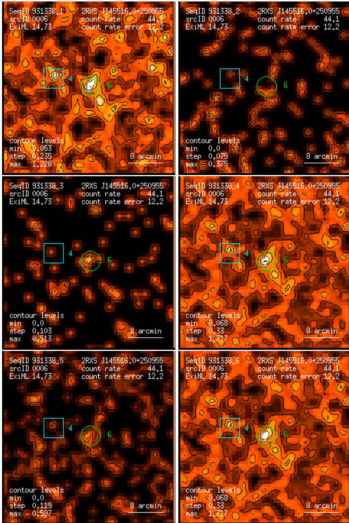
Figure 6: RASS 931338: detection 0006: band rate images, Gaussian filter: (1) PSPC channels 11 – 41, (2) 52 – 90, (3) 91 – 201, (4) 11 – 235, (5) 52 – 201, (6) 11 – 201. Broad band rates in counts/ks. Band rate contour levels in counts/ks/arcmin 2 .
