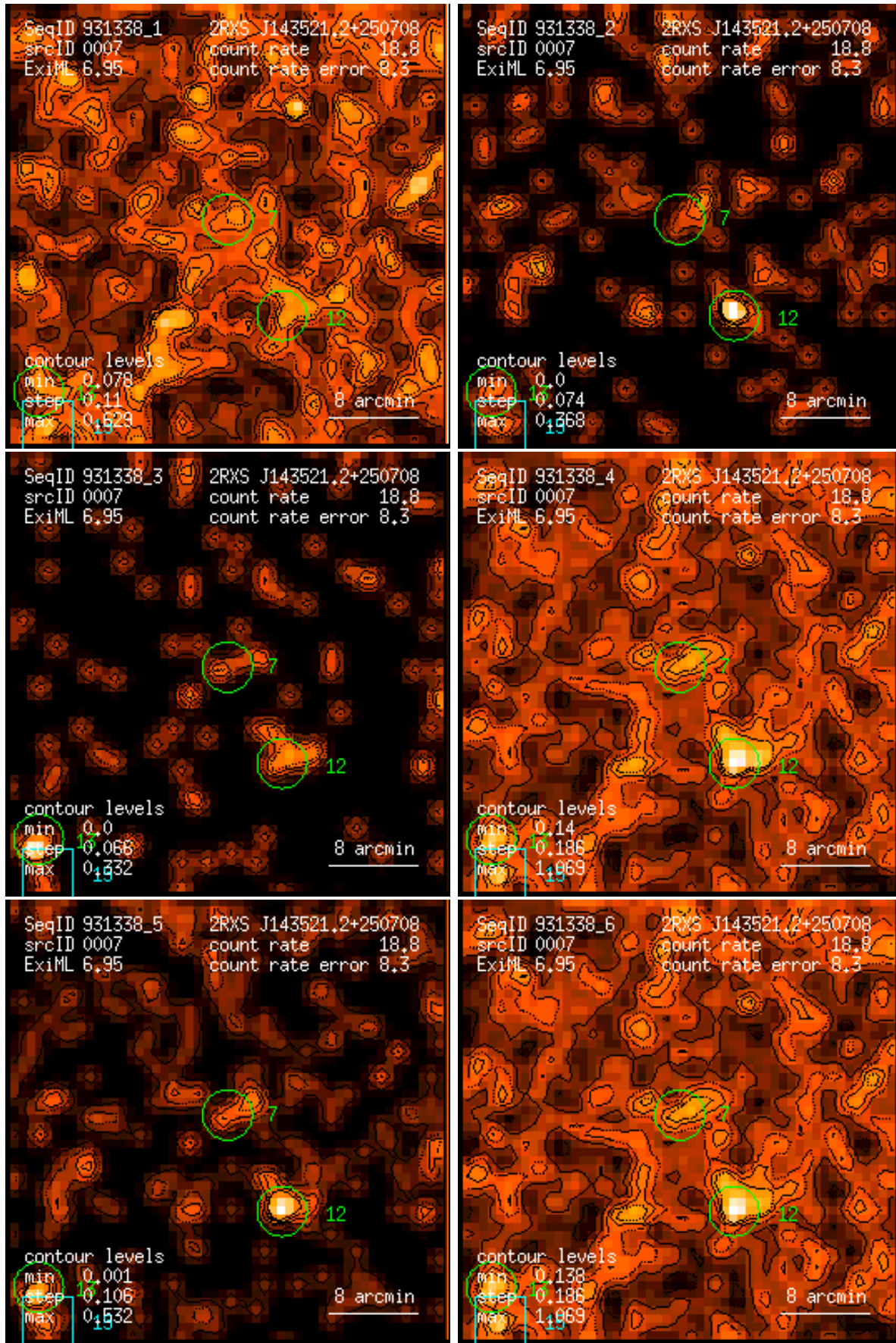
Figure 7: RASS 931338: detection 0007: band rate images, Gaussian filter: (1) PSPC channels 11 – 41, (2) 52 – 90, (3) 91 – 201, (4) 11 – 235, (5) 52 – 201, (6) 11 – 201. Broad band rates in counts/ks. Band rate contour levels in counts/ks/arcmin 2 .
