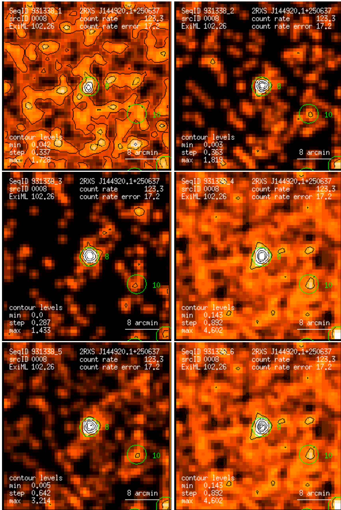
Figure 8: RASS 931338: detection 0008: band rate images, Gaussian filter: (1) PSPC channels 11 – 41, (2) 52 – 90, (3) 91 – 201, (4) 11 – 235, (5) 52 – 201, (6) 11 – 201. Broad band rates in counts/ks. Band rate contour levels in counts/ks/arcmin 2 .
