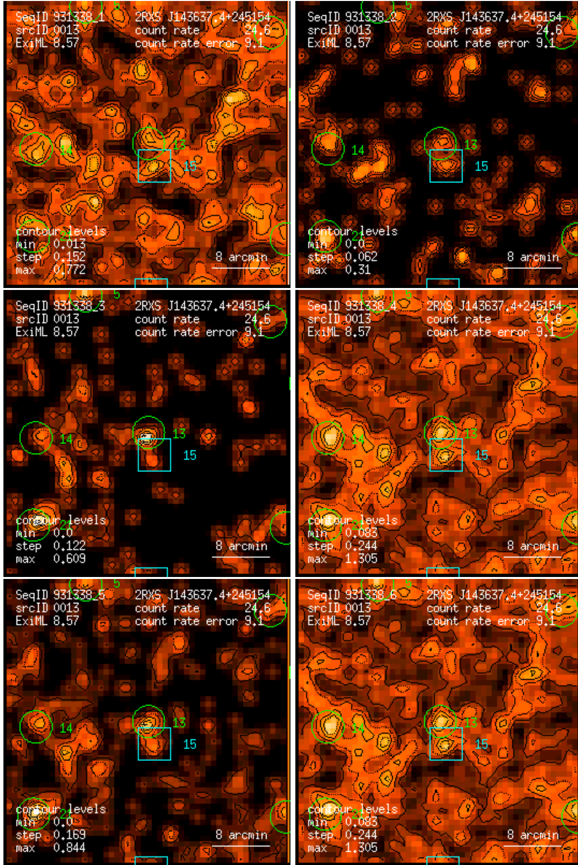
Figure 13: RASS 931338: detection 0013: band rate images, Gaussian filter: (1) PSPC channels 11 – 41, (2) 52 – 90, (3) 91 – 201, (4) 11 – 235, (5) 52 – 201, (6) 11 – 201. Broad band rates in counts/ks. Band rate contour levels in counts/ks/arcmin 2 .
