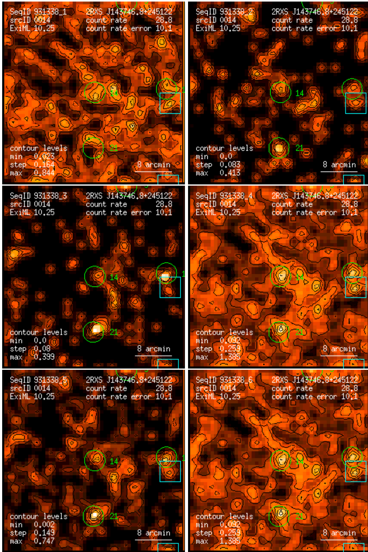
Figure 14: RASS 931338: detection 0014: band rate images, Gaussian filter: (1) PSPC channels 11 – 41, (2) 52 – 90, (3) 91 – 201, (4) 11 – 235, (5) 52 – 201, (6) 11 – 201. Broad band rates in counts/ks. Band rate contour levels in counts/ks/arcmin 2 .
