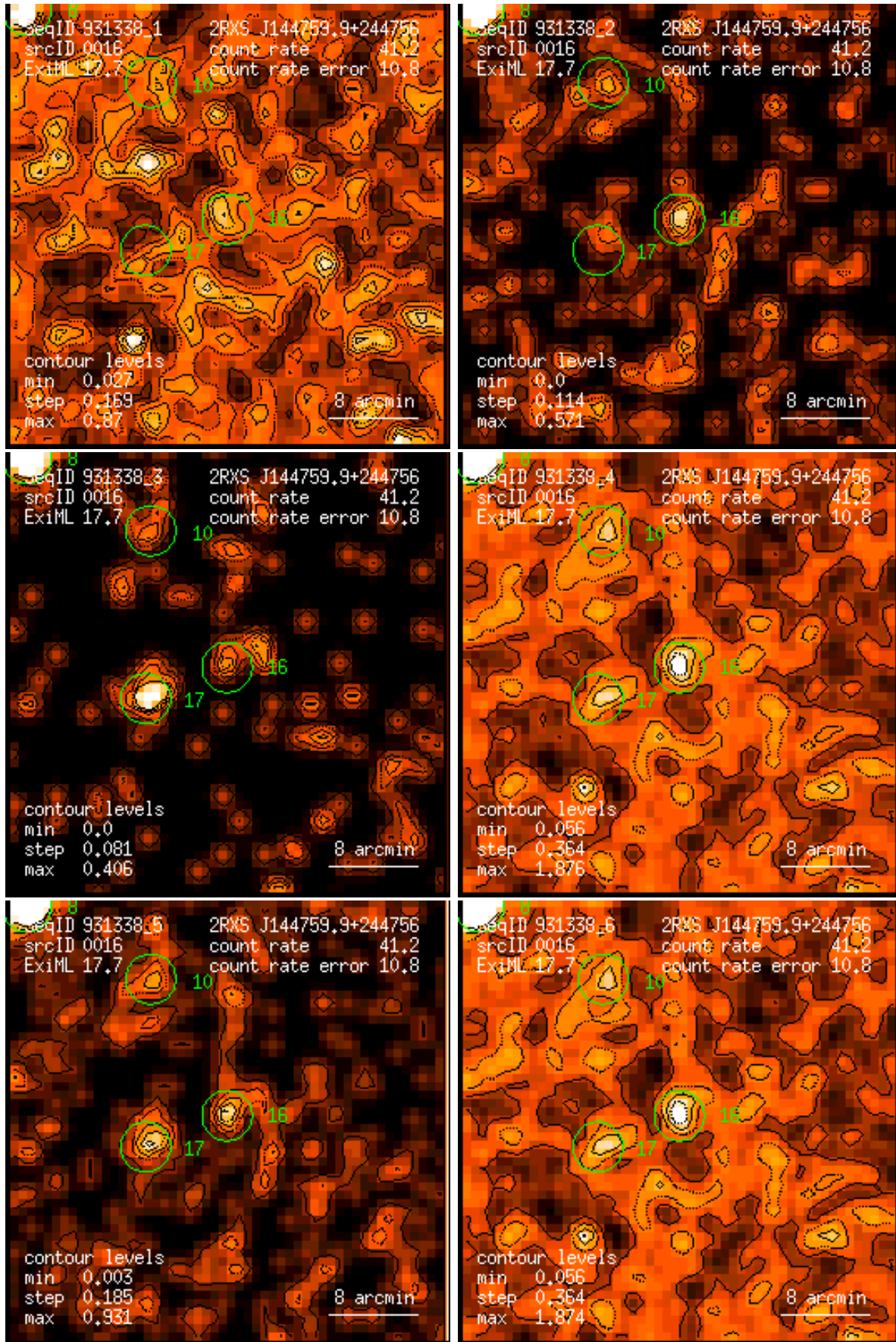
Figure 16: RASS 931338: detection 0016: band rate images, Gaussian filter: (1) PSPC channels 11 – 41, (2) 52 – 90, (3) 91 – 201, (4) 11 – 235, (5) 52 – 201, (6) 11 – 201. Broad band rates in counts/ks. Band rate contour levels in counts/ks/arcmin 2 .
