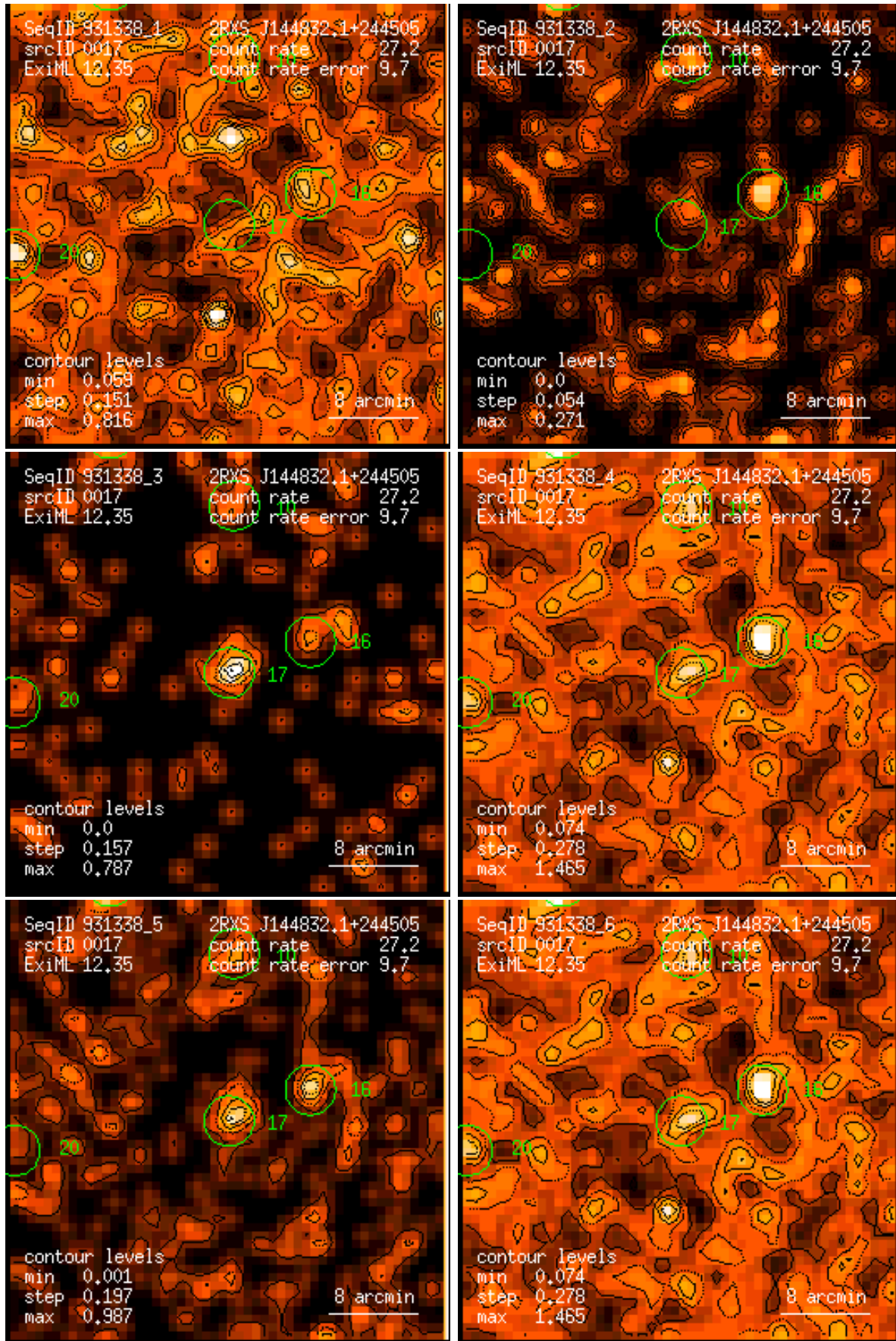
Figure 17: RASS 931338: detection 0017: band rate images, Gaussian filter: (1) PSPC channels 11 – 41, (2) 52 – 90, (3) 91 – 201, (4) 11 – 235, (5) 52 – 201, (6) 11 – 201. Broad band rates in counts/ks. Band rate contour levels in counts/ks/arcmin 2 .
