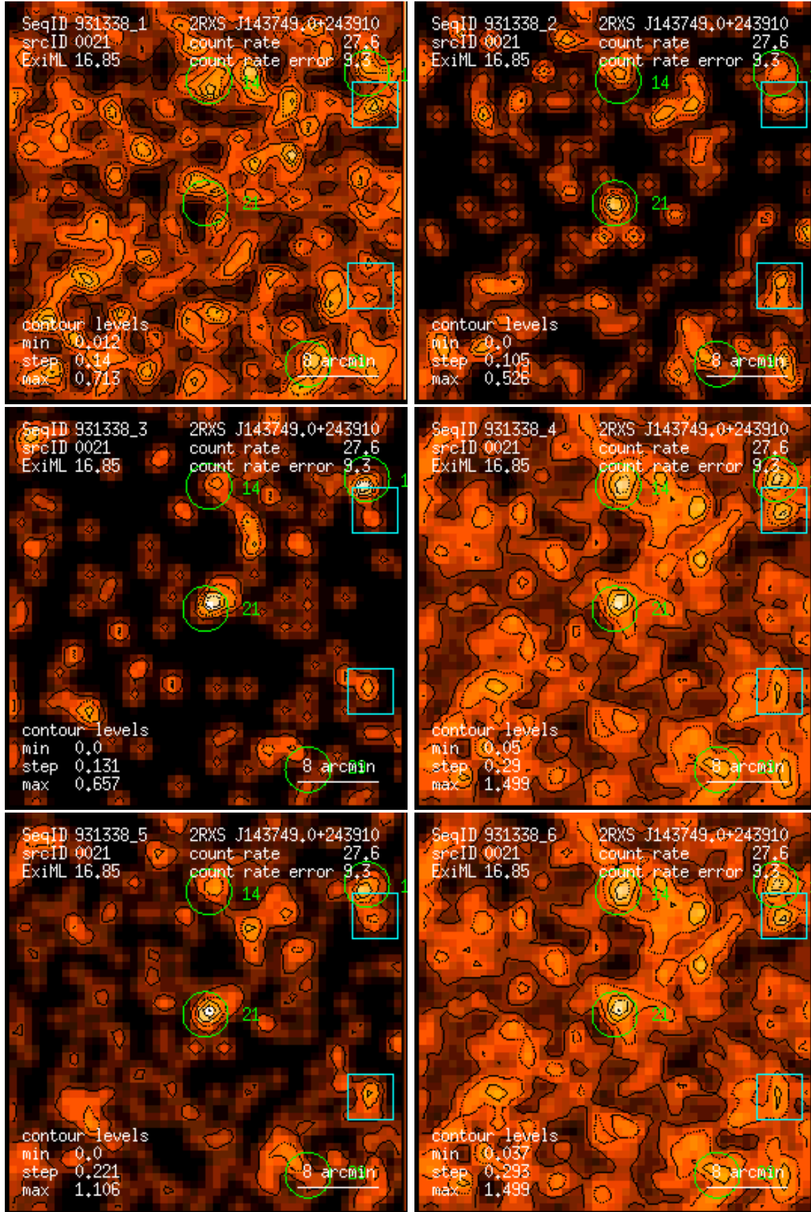
Figure 21: RASS 931338: detection 0021: band rate images, Gaussian filter: (1) PSPC channels 11 – 41, (2) 52 – 90, (3) 91 – 201, (4) 11 – 235, (5) 52 – 201, (6) 11 – 201. Broad band rates in counts/ks. Band rate contour levels in counts/ks/arcmin 2 .
