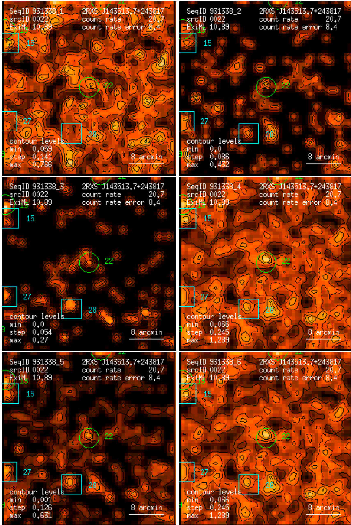
Figure 22: RASS 931338: detection 0022: band rate images, Gaussian filter: (1) PSPC channels 11 – 41, (2) 52 – 90, (3) 91 – 201, (4) 11 – 235, (5) 52 – 201, (6) 11 – 201. Broad band rates in counts/ks. Band rate contour levels in counts/ks/arcmin 2 .
