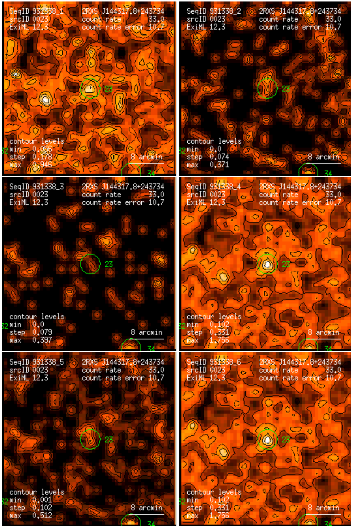
Figure 23: RASS 931338: detection 0023: band rate images, Gaussian filter: (1) PSPC channels 11 – 41, (2) 52 – 90, (3) 91 – 201, (4) 11 – 235, (5) 52 – 201, (6) 11 – 201. Broad band rates in counts/ks. Band rate contour levels in counts/ks/arcmin 2 .
