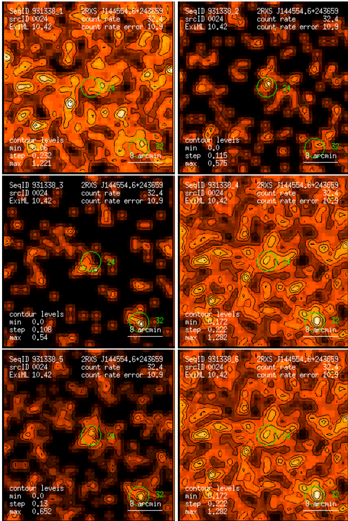
Figure 24: RASS 931338: detection 0024: band rate images, Gaussian filter: (1) PSPC channels 11 – 41, (2) 52 – 90, (3) 91 – 201, (4) 11 – 235, (5) 52 – 201, (6) 11 – 201. Broad band rates in counts/ks. Band rate contour levels in counts/ks/arcmin 2 .
