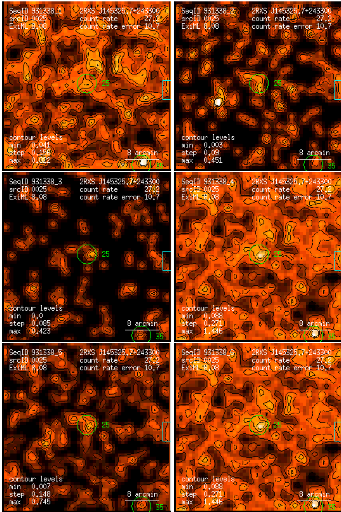
Figure 25: RASS 931338: detection 0025: band rate images, Gaussian filter: (1) PSPC channels 11 – 41, (2) 52 – 90, (3) 91 – 201, (4) 11 – 235, (5) 52 – 201, (6) 11 – 201. Broad band rates in counts/ks. Band rate contour levels in counts/ks/arcmin 2 .
