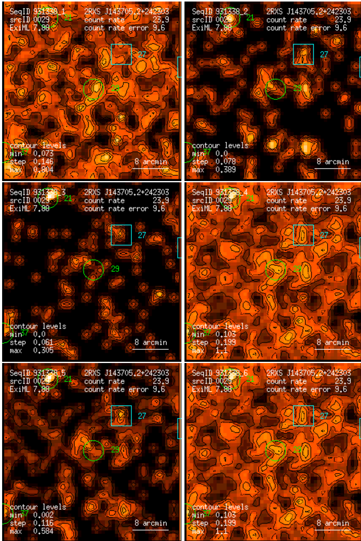
Figure 29: RASS 931338: detection 0029: band rate images, Gaussian filter: (1) PSPC channels 11 – 41, (2) 52 – 90, (3) 91 – 201, (4) 11 – 235, (5) 52 – 201, (6) 11 – 201. Broad band rates in counts/ks. Band rate contour levels in counts/ks/arcmin 2 .
