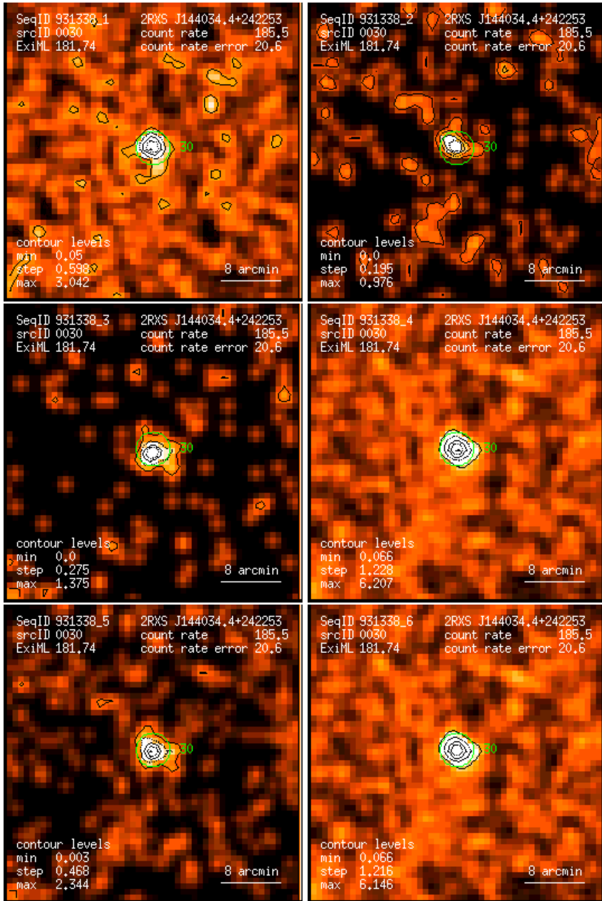
Figure 30: RASS 931338: detection 0030: band rate images, Gaussian filter: (1) PSPC channels 11 – 41, (2) 52 – 90, (3) 91 – 201, (4) 11 – 235, (5) 52 – 201, (6) 11 – 201. Broad band rates in counts/ks. Band rate contour levels in counts/ks/arcmin 2 .
