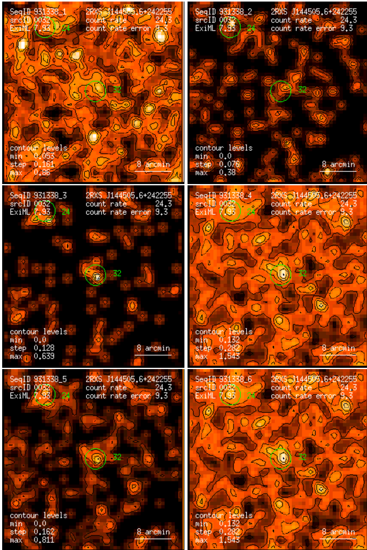
Figure 32: RASS 931338: detection 0032: band rate images, Gaussian filter: (1) PSPC channels 11 – 41, (2) 52 – 90, (3) 91 – 201, (4) 11 – 235, (5) 52 – 201, (6) 11 – 201. Broad band rates in counts/ks. Band rate contour levels in counts/ks/arcmin 2 .
