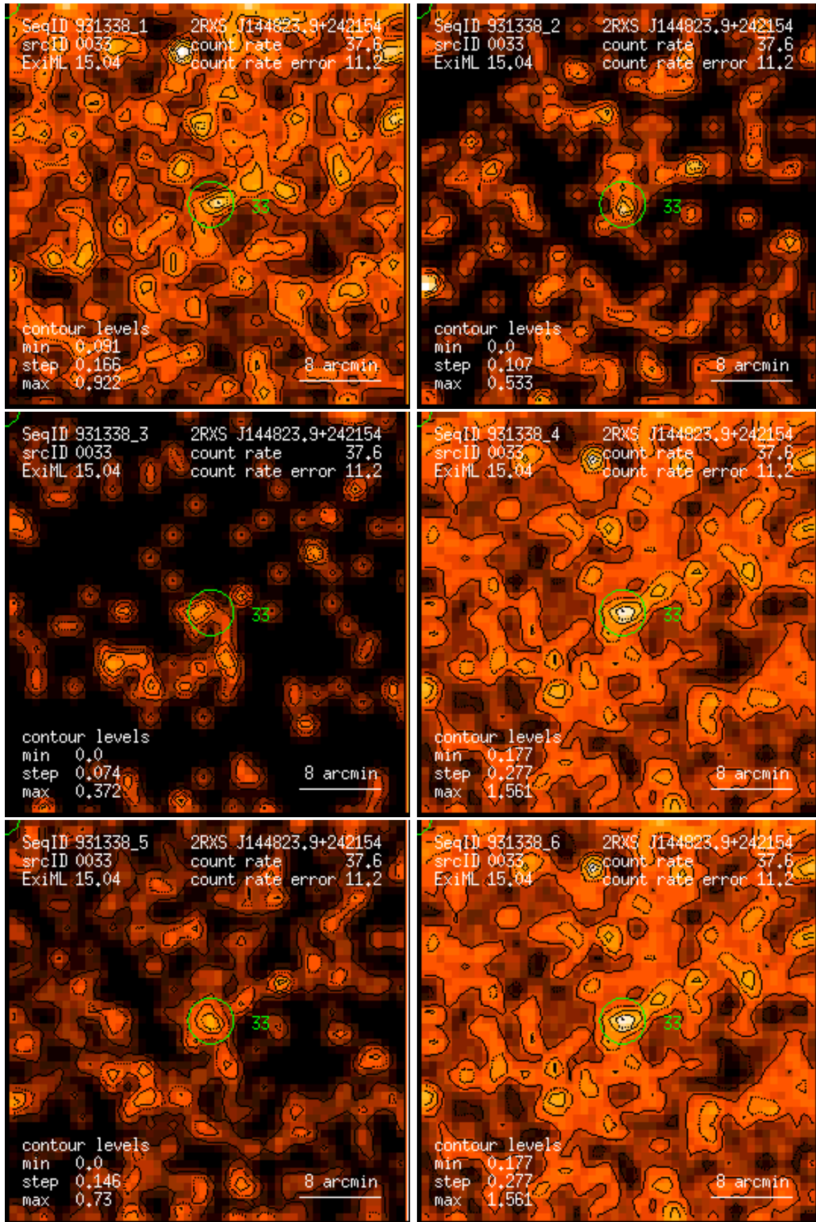
Figure 33: RASS 931338: detection 0033: band rate images, Gaussian filter: (1) PSPC channels 11 – 41, (2) 52 – 90, (3) 91 – 201, (4) 11 – 235, (5) 52 – 201, (6) 11 – 201. Broad band rates in counts/ks. Band rate contour levels in counts/ks/arcmin 2 .
