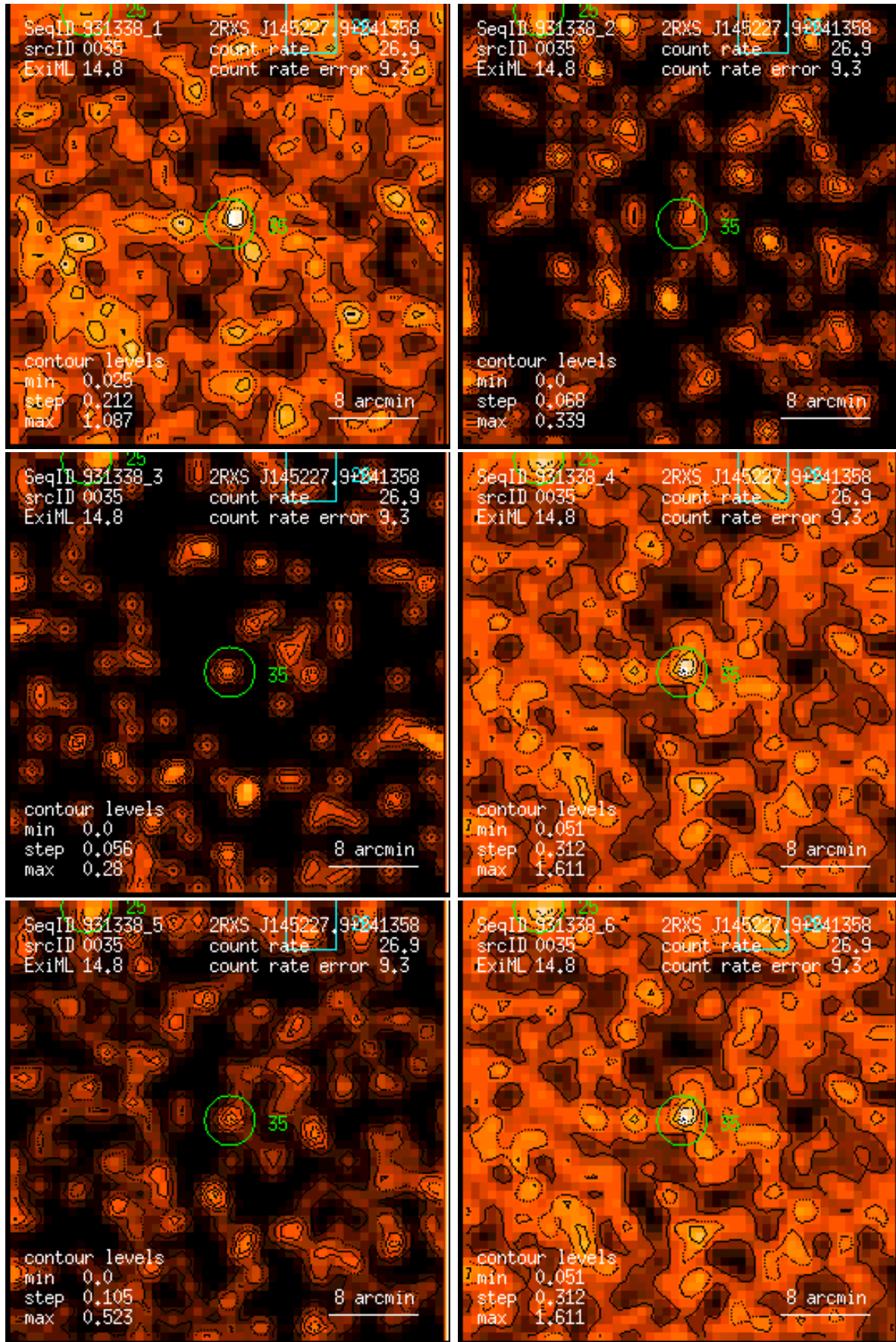
Figure 35: RASS 931338: detection 0035: band rate images, Gaussian filter: (1) PSPC channels 11 – 41, (2) 52 – 90, (3) 91 – 201, (4) 11 – 235, (5) 52 – 201, (6) 11 – 201. Broad band rates in counts/ks. Band rate contour levels in counts/ks/arcmin 2 .
