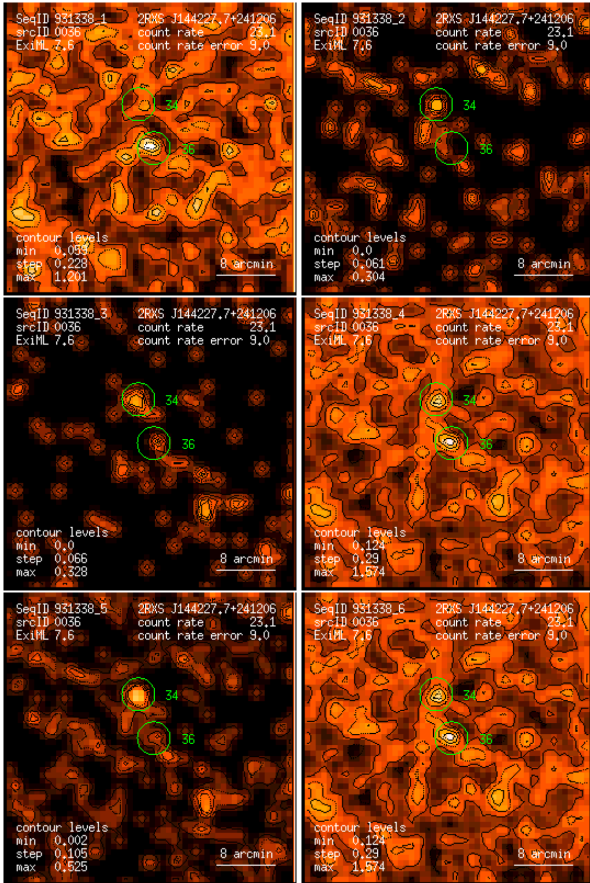
Figure 36: RASS 931338: detection 0036: band rate images, Gaussian filter: (1) PSPC channels 11 – 41, (2) 52 – 90, (3) 91 – 201, (4) 11 – 235, (5) 52 – 201, (6) 11 – 201. Broad band rates in counts/ks. Band rate contour levels in counts/ks/arcmin 2 .
