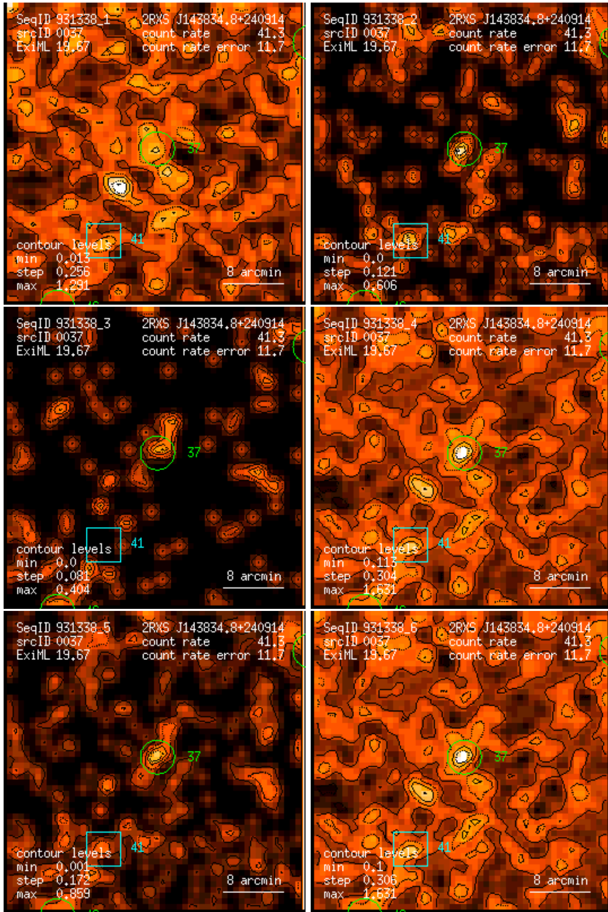
Figure 37: RASS 931338: detection 0037: band rate images, Gaussian filter: (1) PSPC channels 11 – 41, (2) 52 – 90, (3) 91 – 201, (4) 11 – 235, (5) 52 – 201, (6) 11 – 201. Broad band rates in counts/ks. Band rate contour levels in counts/ks/arcmin 2 .
