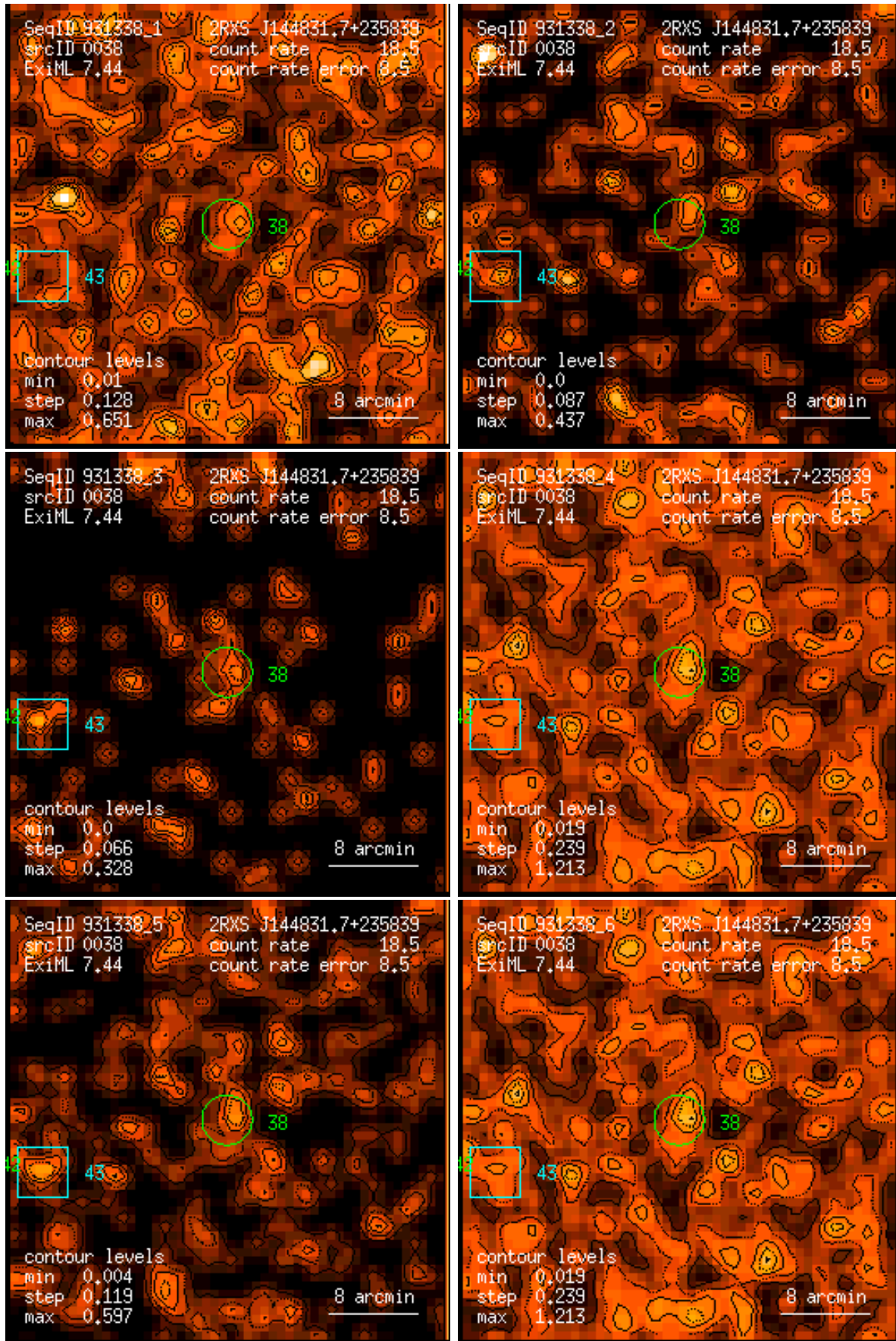
Figure 38: RASS 931338: detection 0038: band rate images, Gaussian filter: (1) PSPC channels 11 – 41, (2) 52 – 90, (3) 91 – 201, (4) 11 – 235, (5) 52 – 201, (6) 11 – 201. Broad band rates in counts/ks. Band rate contour levels in counts/ks/arcmin 2 .
