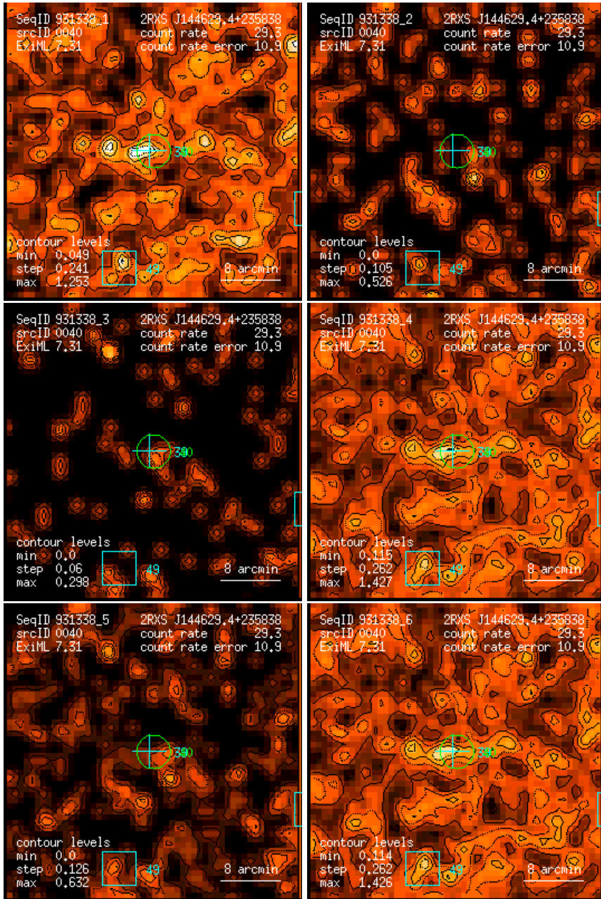
Figure 40: RASS 931338: detection 0040: band rate images, Gaussian filter: (1) PSPC channels 11 – 41, (2) 52 – 90, (3) 91 – 201, (4) 11 – 235, (5) 52 – 201, (6) 11 – 201. Broad band rates in counts/ks. Band rate contour levels in counts/ks/arcmin 2 .
