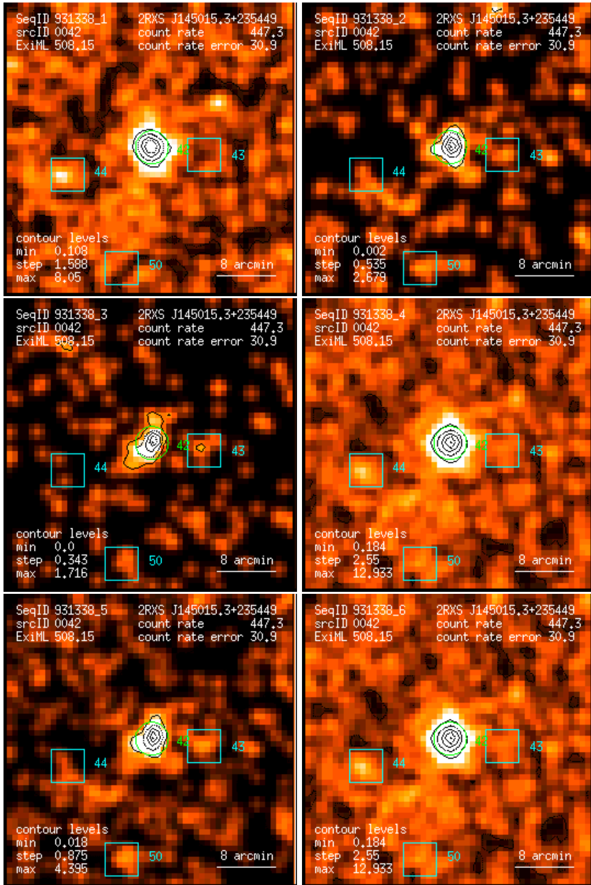
Figure 42: RASS 931338: detection 0042: band rate images, Gaussian filter: (1) PSPC channels 11 – 41, (2) 52 – 90, (3) 91 – 201, (4) 11 – 235, (5) 52 – 201, (6) 11 – 201. Broad band rates in counts/ks. Band rate contour levels in counts/ks/arcmin 2 .
