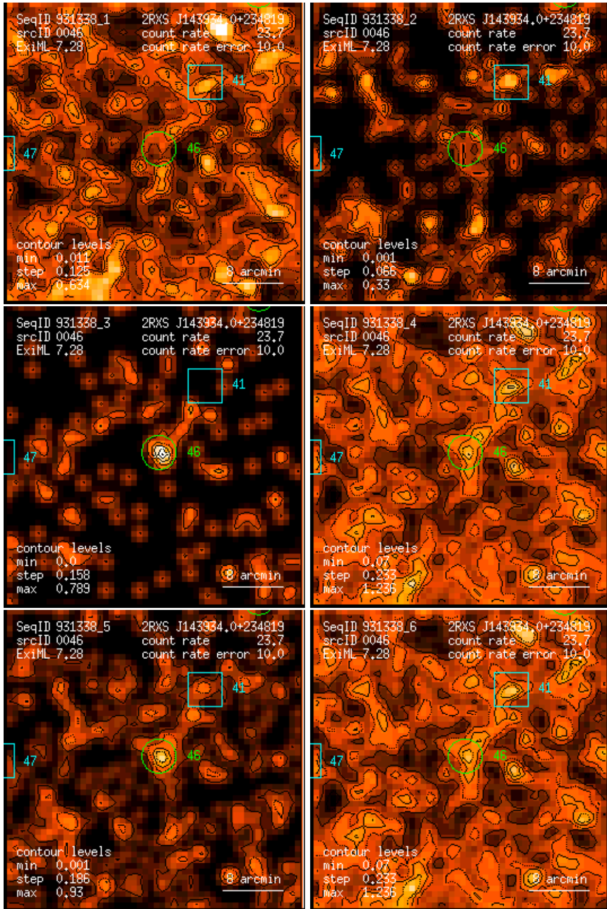
Figure 46: RASS 931338: detection 0046: band rate images, Gaussian filter: (1) PSPC channels 11 – 41, (2) 52 – 90, (3) 91 – 201, (4) 11 – 235, (5) 52 – 201, (6) 11 – 201. Broad band rates in counts/ks. Band rate contour levels in counts/ks/arcmin 2 .
