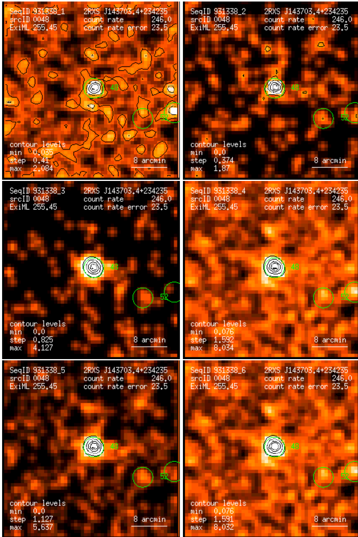
Figure 48: RASS 931338: detection 0048: band rate images, Gaussian filter: (1) PSPC channels 11 – 41, (2) 52 – 90, (3) 91 – 201, (4) 11 – 235, (5) 52 – 201, (6) 11 – 201. Broad band rates in counts/ks. Band rate contour levels in counts/ks/arcmin 2 .
