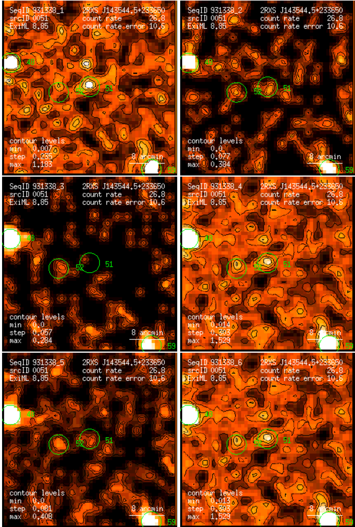
Figure 51: RASS 931338: detection 0051: band rate images, Gaussian filter: (1) PSPC channels 11 – 41, (2) 52 – 90, (3) 91 – 201, (4) 11 – 235, (5) 52 – 201, (6) 11 – 201. Broad band rates in counts/ks. Band rate contour levels in counts/ks/arcmin 2 .
