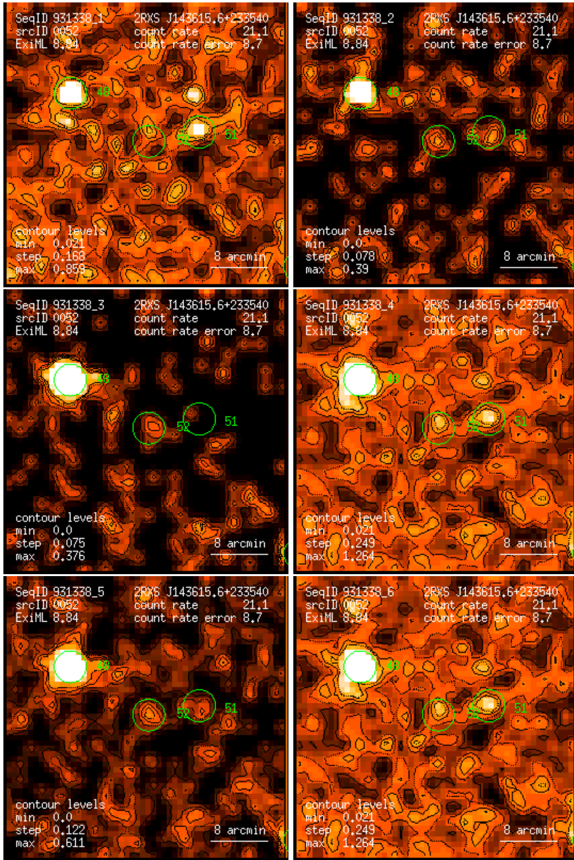
Figure 52: RASS 931338: detection 0052: band rate images, Gaussian filter: (1) PSPC channels 11 – 41, (2) 52 – 90, (3) 91 – 201, (4) 11 – 235, (5) 52 – 201, (6) 11 – 201. Broad band rates in counts/ks. Band rate contour levels in counts/ks/arcmin 2 .
