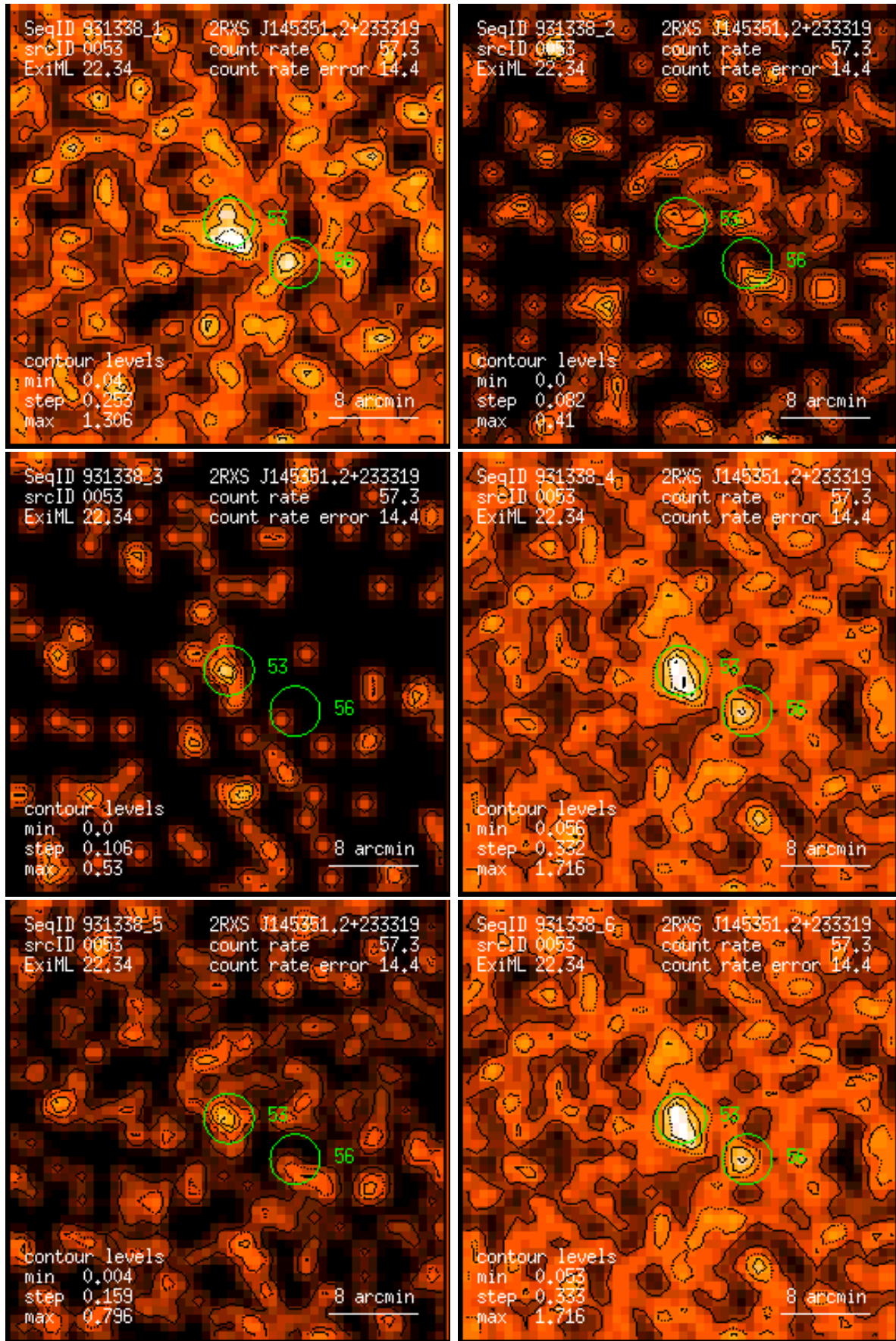
Figure 53: RASS 931338: detection 0053: band rate images, Gaussian filter: (1) PSPC channels 11 – 41, (2) 52 – 90, (3) 91 – 201, (4) 11 – 235, (5) 52 – 201, (6) 11 – 201. Broad band rates in counts/ks. Band rate contour levels in counts/ks/arcmin 2 .
