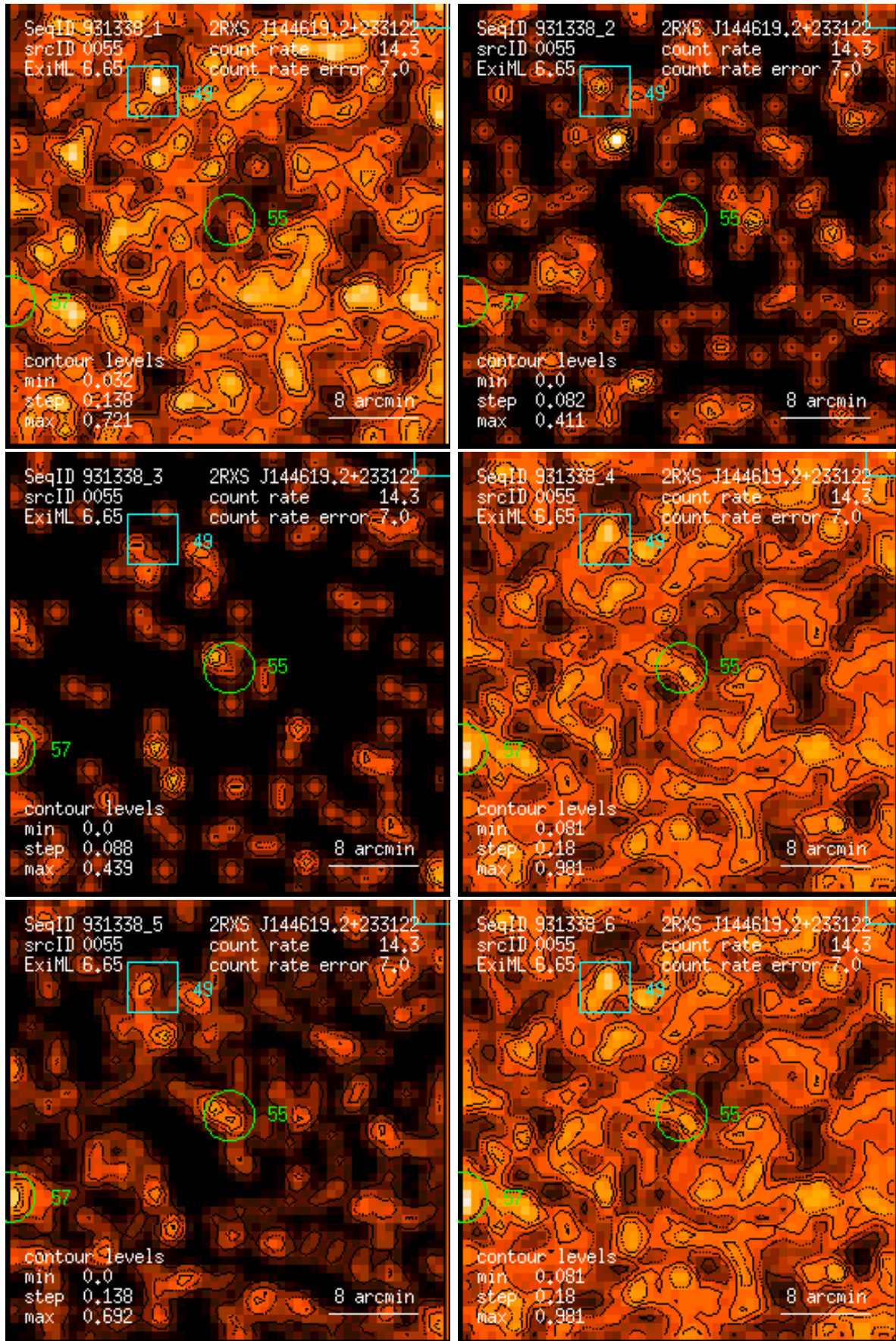
Figure 55: RASS 931338: detection 0055: band rate images, Gaussian filter: (1) PSPC channels 11 – 41, (2) 52 – 90, (3) 91 – 201, (4) 11 – 235, (5) 52 – 201, (6) 11 – 201. Broad band rates in counts/ks. Band rate contour levels in counts/ks/arcmin 2 .
