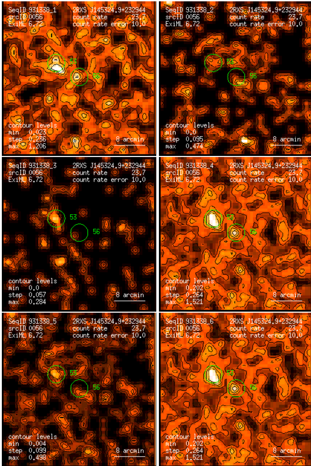
Figure 56: RASS 931338: detection 0056: band rate images, Gaussian filter: (1) PSPC channels 11 – 41, (2) 52 – 90, (3) 91 – 201, (4) 11 – 235, (5) 52 – 201, (6) 11 – 201. Broad band rates in counts/ks. Band rate contour levels in counts/ks/arcmin 2 .
