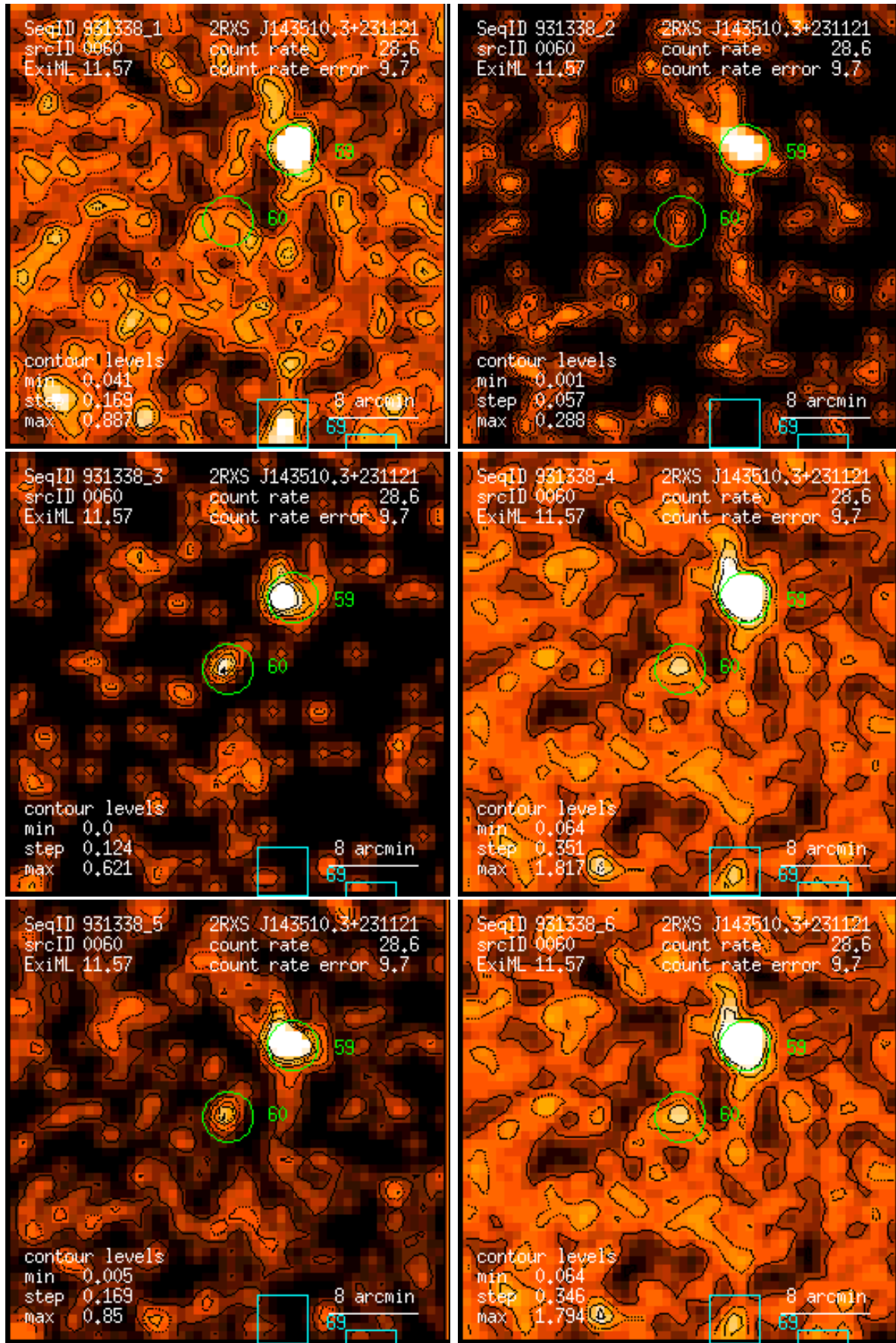
Figure 60: RASS 931338: detection 0060: band rate images, Gaussian filter: (1) PSPC channels 11 – 41, (2) 52 – 90, (3) 91 – 201, (4) 11 – 235, (5) 52 – 201, (6) 11 – 201. Broad band rates in counts/ks. Band rate contour levels in counts/ks/arcmin 2 .
