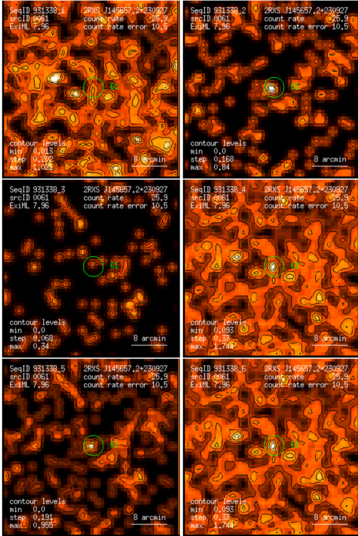
Figure 61: RASS 931338: detection 0061: band rate images, Gaussian filter: (1) PSPC channels 11 – 41, (2) 52 – 90, (3) 91 – 201, (4) 11 – 235, (5) 52 – 201, (6) 11 – 201. Broad band rates in counts/ks. Band rate contour levels in counts/ks/arcmin 2 .
