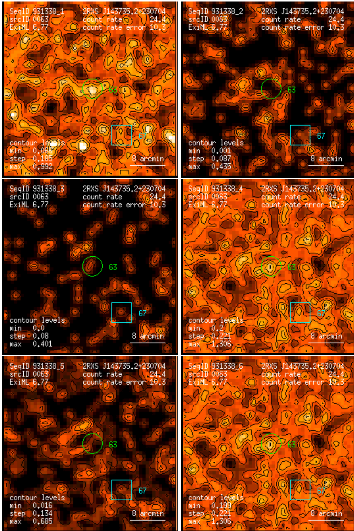
Figure 63: RASS 931338: detection 0063: band rate images, Gaussian filter: (1) PSPC channels 11 – 41, (2) 52 – 90, (3) 91 – 201, (4) 11 – 235, (5) 52 – 201, (6) 11 – 201. Broad band rates in counts/ks. Band rate contour levels in counts/ks/arcmin 2 .
