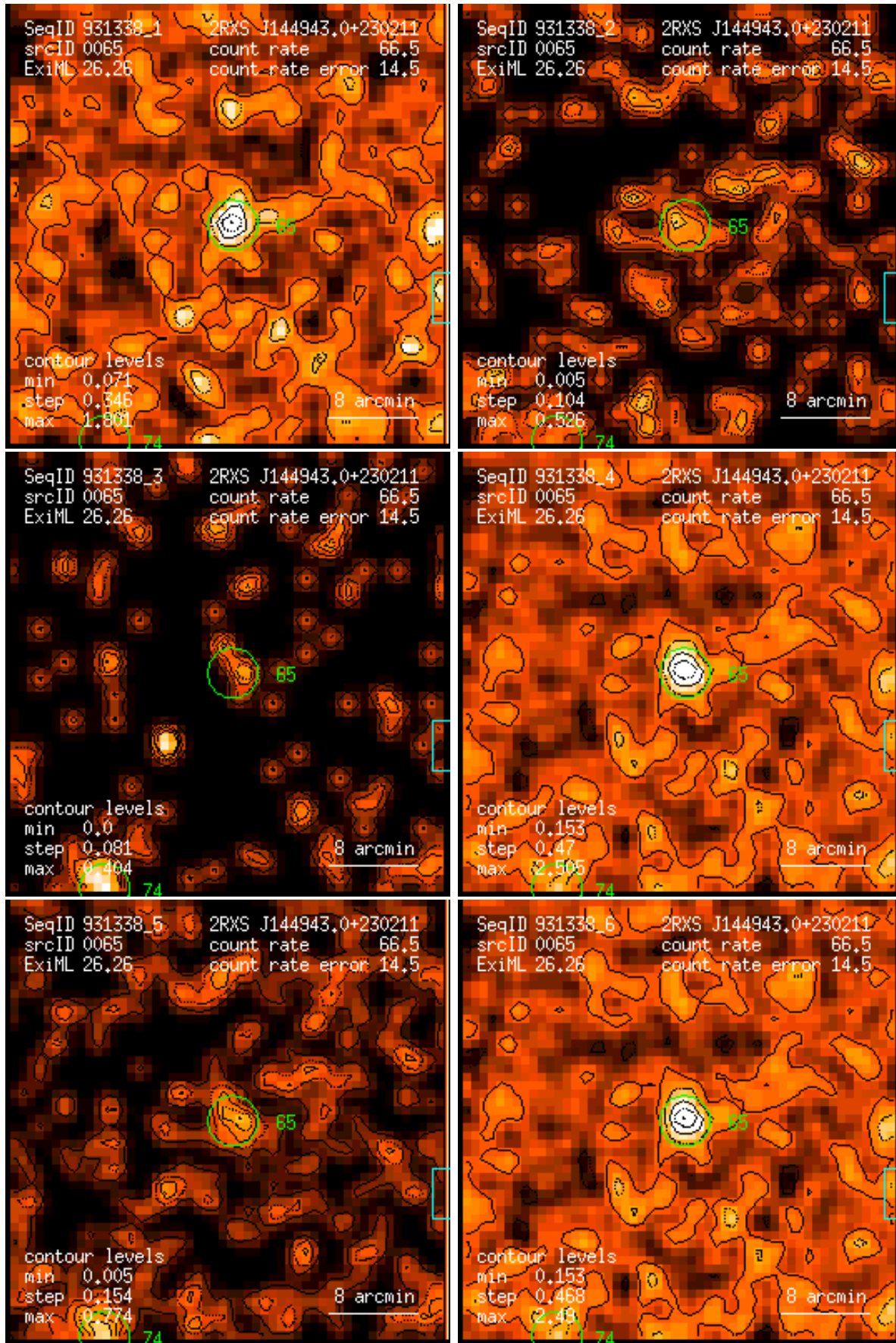
Figure 65: RASS 931338: detection 0065: band rate images, Gaussian filter: (1) PSPC channels 11 – 41, (2) 52 – 90, (3) 91 – 201, (4) 11 – 235, (5) 52 – 201, (6) 11 – 201. Broad band rates in counts/ks. Band rate contour levels in counts/ks/arcmin 2 .
