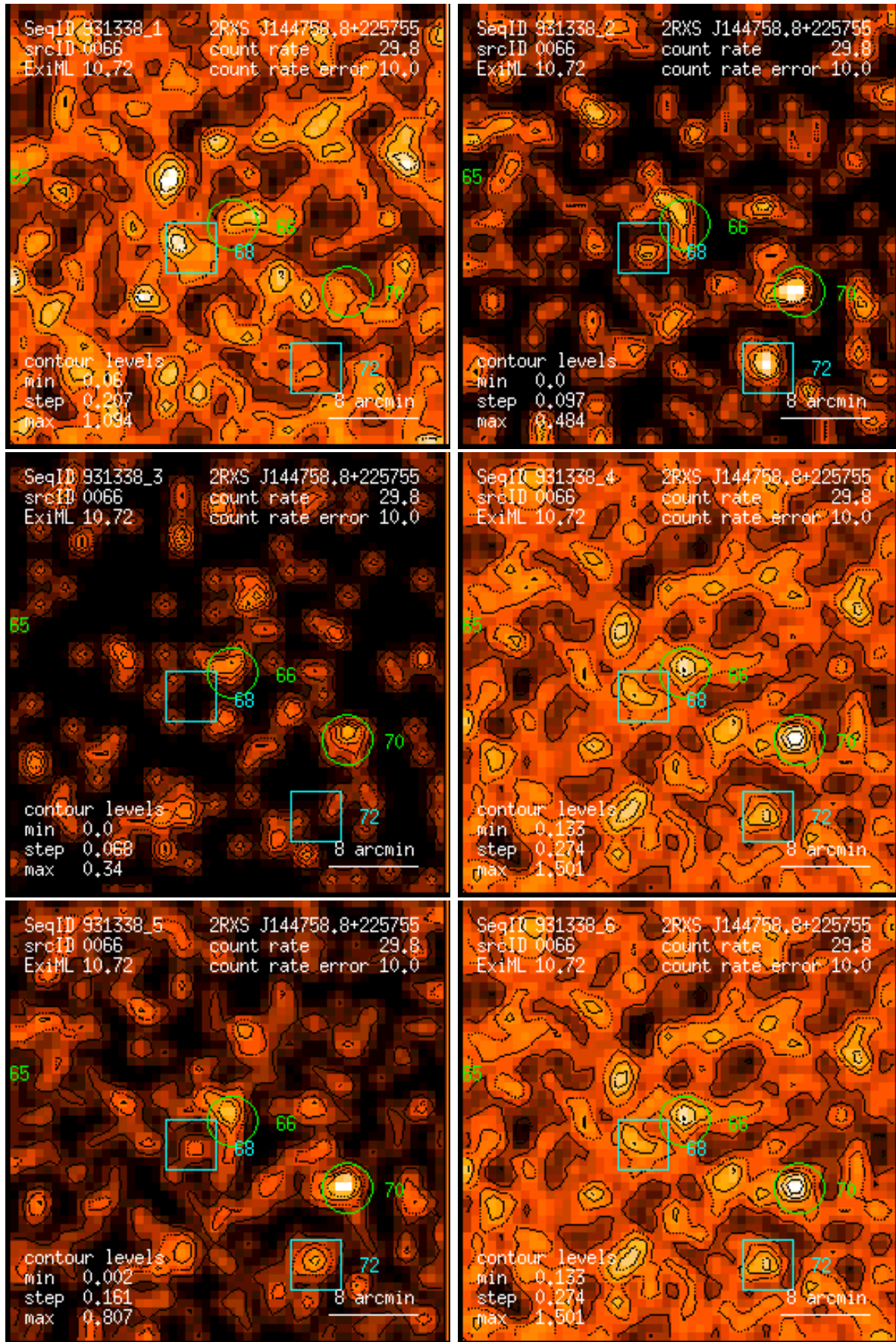
Figure 66: RASS 931338: detection 0066: band rate images, Gaussian filter: (1) PSPC channels 11 – 41, (2) 52 – 90, (3) 91 – 201, (4) 11 – 235, (5) 52 – 201, (6) 11 – 201. Broad band rates in counts/ks. Band rate contour levels in counts/ks/arcmin 2 .
