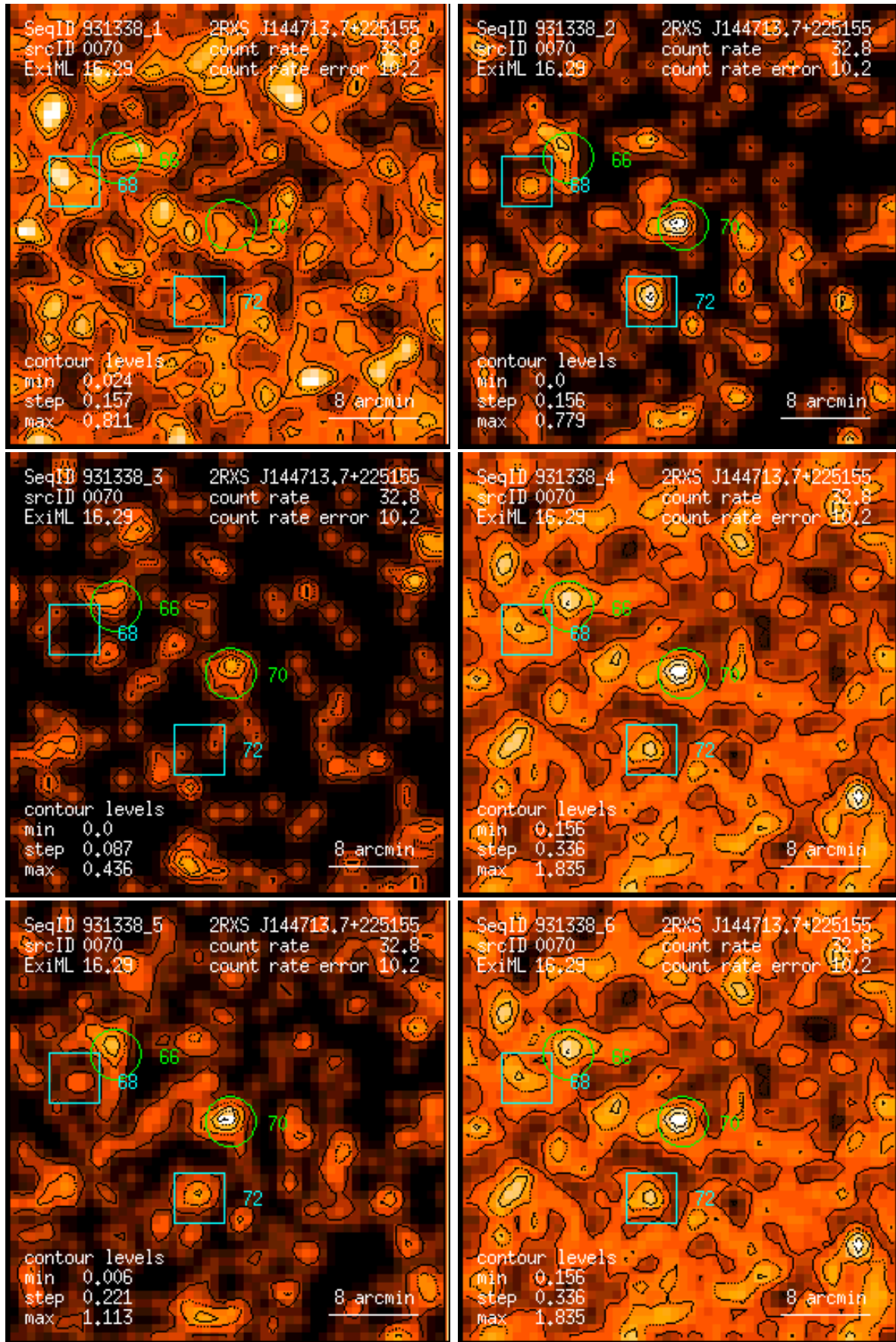
Figure 70: RASS 931338: detection 0070: band rate images, Gaussian filter: (1) PSPC channels 11 – 41, (2) 52 – 90, (3) 91 – 201, (4) 11 – 235, (5) 52 – 201, (6) 11 – 201. Broad band rates in counts/ks. Band rate contour levels in counts/ks/arcmin 2 .
