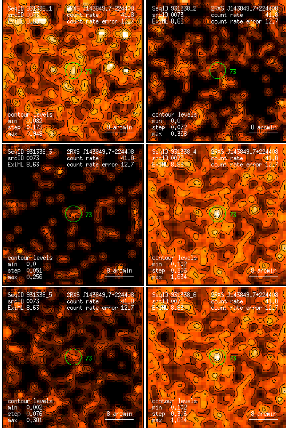
Figure 73: RASS 931338: detection 0073: band rate images, Gaussian filter: (1) PSPC channels 11 – 41, (2) 52 – 90, (3) 91 – 201, (4) 11 – 235, (5) 52 – 201, (6) 11 – 201. Broad band rates in counts/ks. Band rate contour levels in counts/ks/arcmin 2 .
