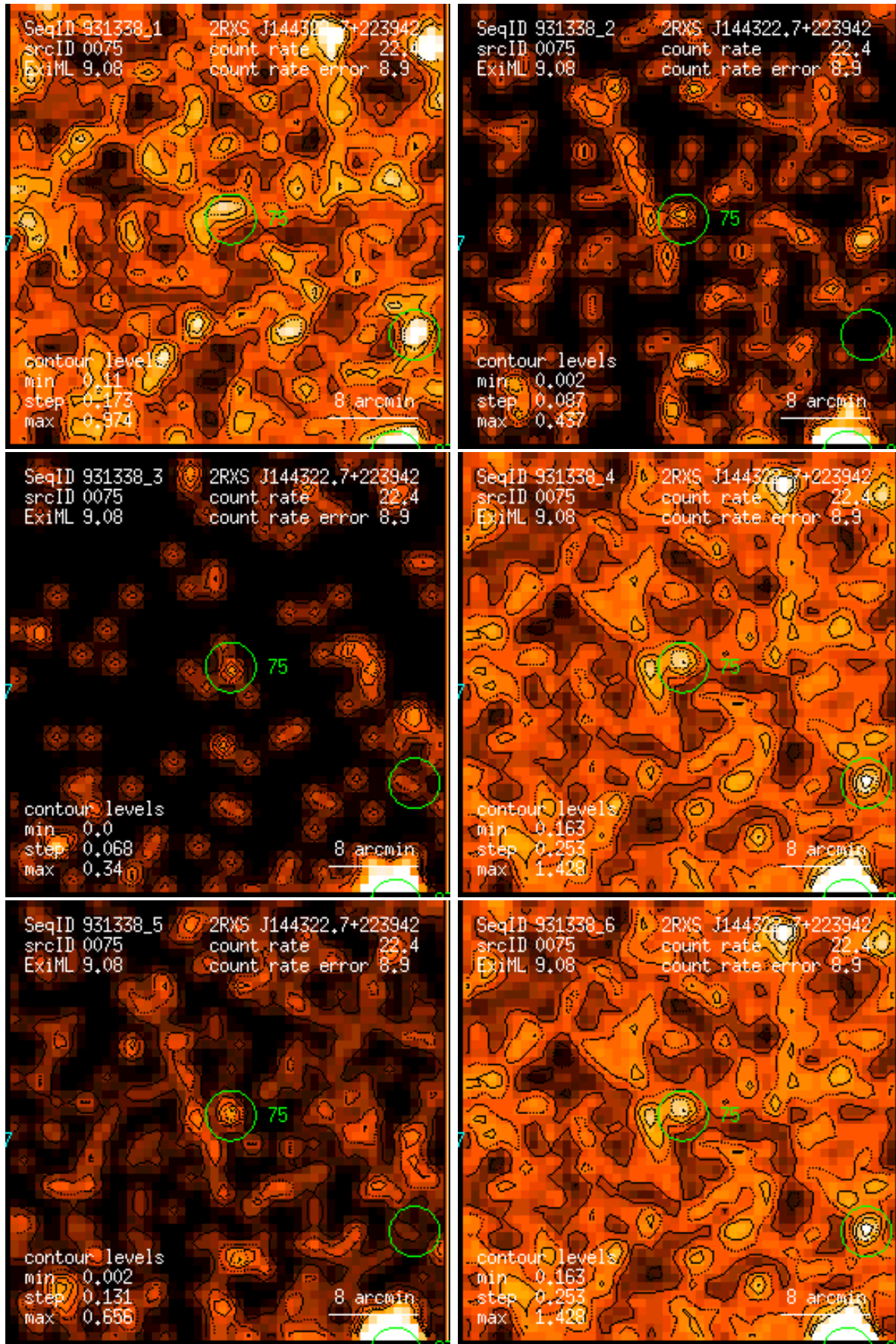
Figure 75: RASS 931338: detection 0075: band rate images, Gaussian filter: (1) PSPC channels 11 – 41, (2) 52 – 90, (3) 91 – 201, (4) 11 – 235, (5) 52 – 201, (6) 11 – 201. Broad band rates in counts/ks. Band rate contour levels in counts/ks/arcmin 2 .
