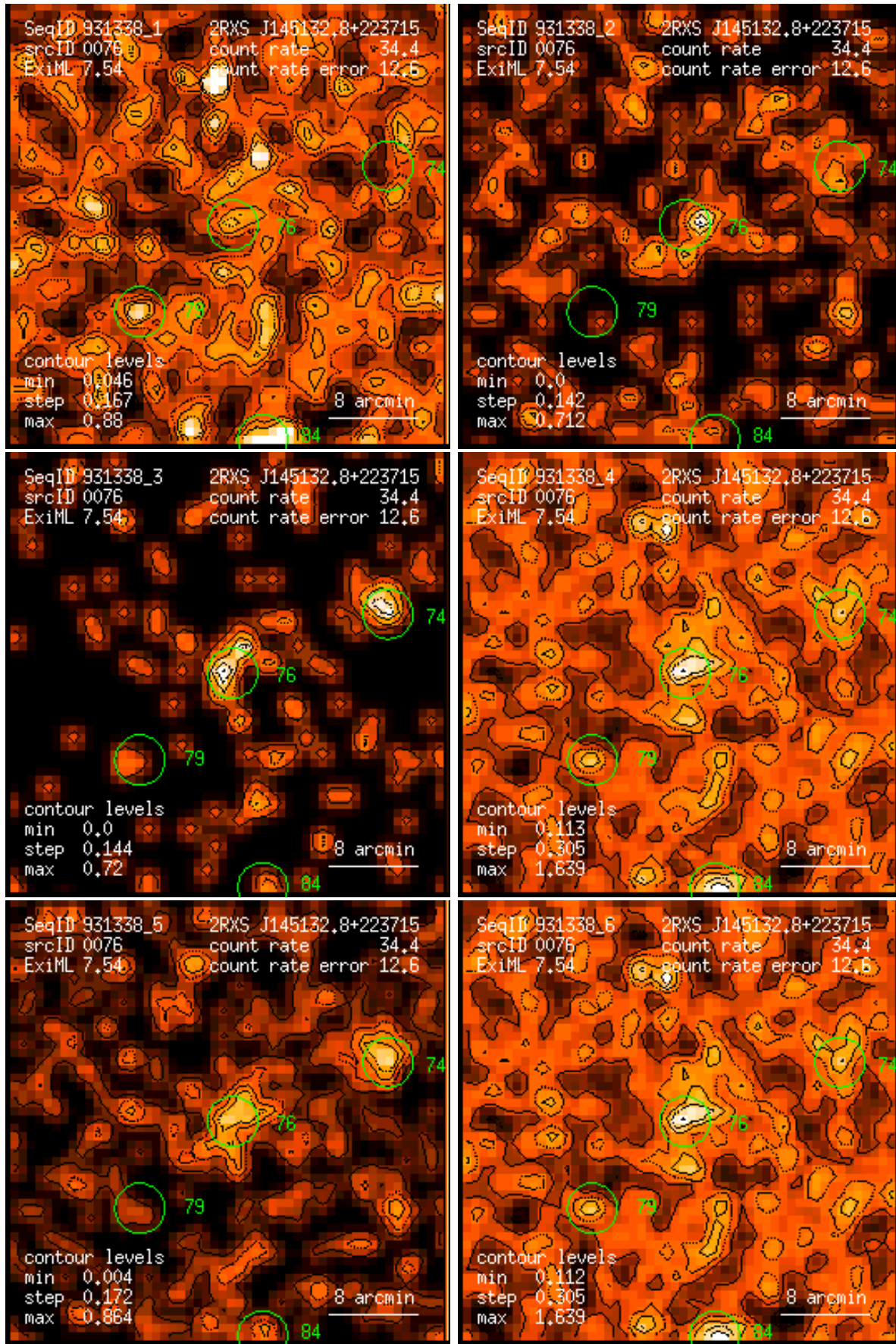
Figure 76: RASS 931338: detection 0076: band rate images, Gaussian filter: (1) PSPC channels 11 – 41, (2) 52 – 90, (3) 91 – 201, (4) 11 – 235, (5) 52 – 201, (6) 11 – 201. Broad band rates in counts/ks. Band rate contour levels in counts/ks/arcmin 2 .
