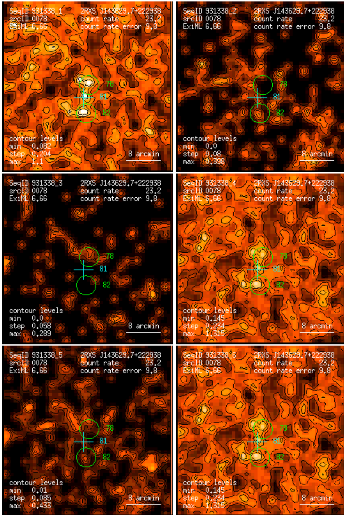
Figure 78: RASS 931338: detection 0078: band rate images, Gaussian filter: (1) PSPC channels 11 – 41, (2) 52 – 90, (3) 91 – 201, (4) 11 – 235, (5) 52 – 201, (6) 11 – 201. Broad band rates in counts/ks. Band rate contour levels in counts/ks/arcmin 2 .
