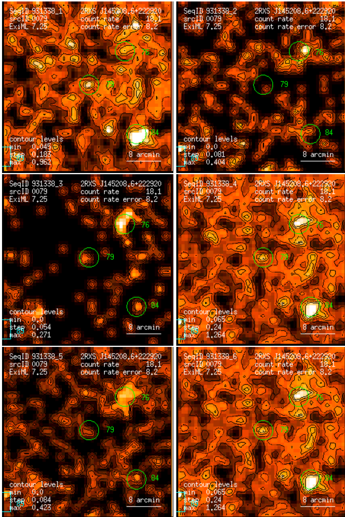
Figure 79: RASS 931338: detection 0079: band rate images, Gaussian filter: (1) PSPC channels 11 – 41, (2) 52 – 90, (3) 91 – 201, (4) 11 – 235, (5) 52 – 201, (6) 11 – 201. Broad band rates in counts/ks. Band rate contour levels in counts/ks/arcmin 2 .
