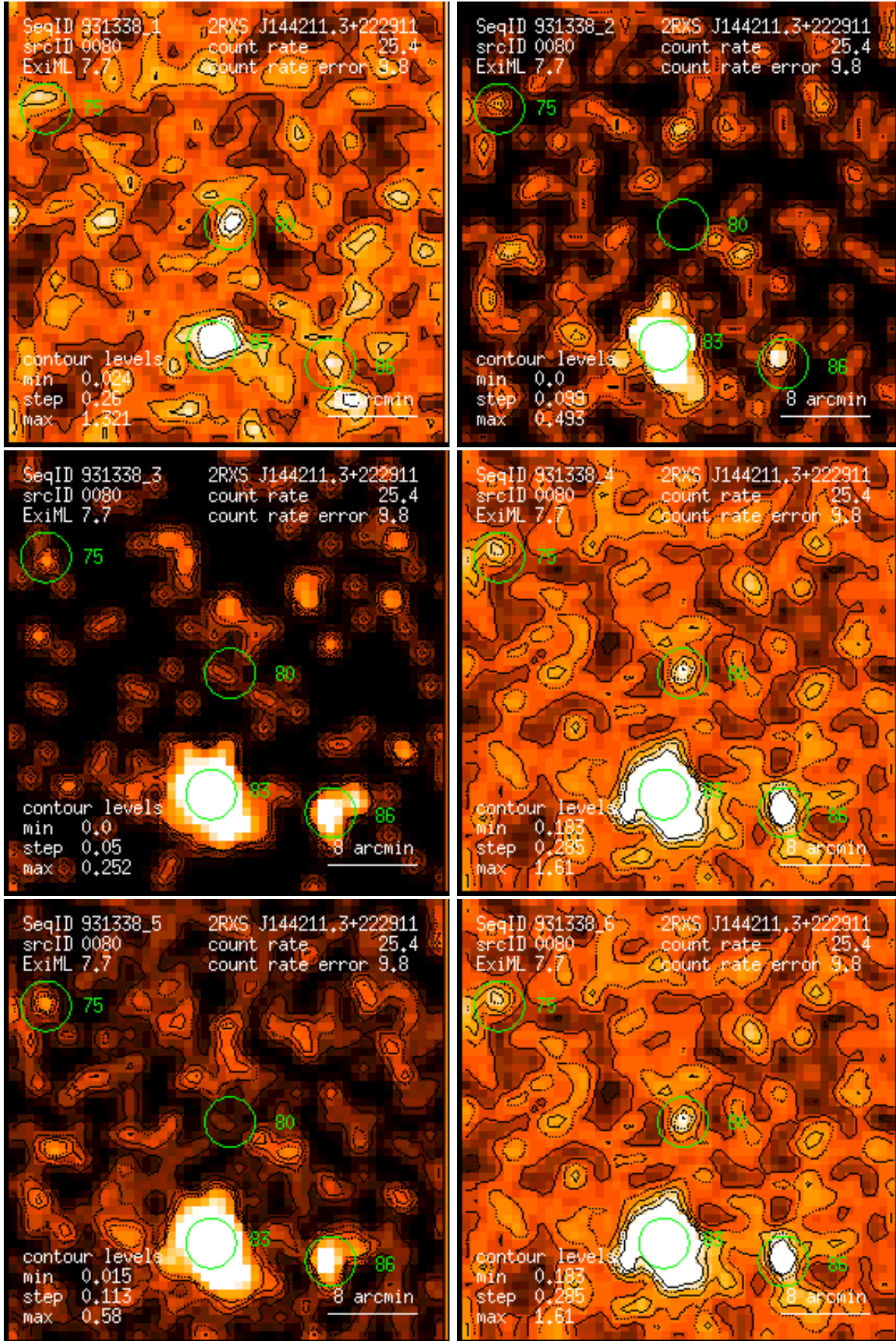
Figure 80: RASS 931338: detection 0080: band rate images, Gaussian filter: (1) PSPC channels 11 – 41, (2) 52 – 90, (3) 91 – 201, (4) 11 – 235, (5) 52 – 201, (6) 11 – 201. Broad band rates in counts/ks. Band rate contour levels in counts/ks/arcmin 2 .
