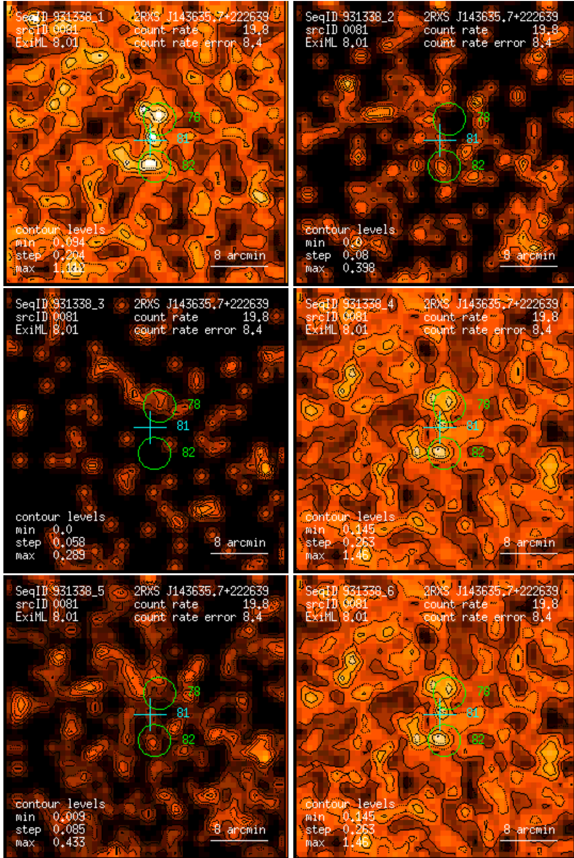
Figure 81: RASS 931338: detection 0081: band rate images, Gaussian filter: (1) PSPC channels 11 – 41, (2) 52 – 90, (3) 91 – 201, (4) 11 – 235, (5) 52 – 201, (6) 11 – 201. Broad band rates in counts/ks. Band rate contour levels in counts/ks/arcmin 2 .
