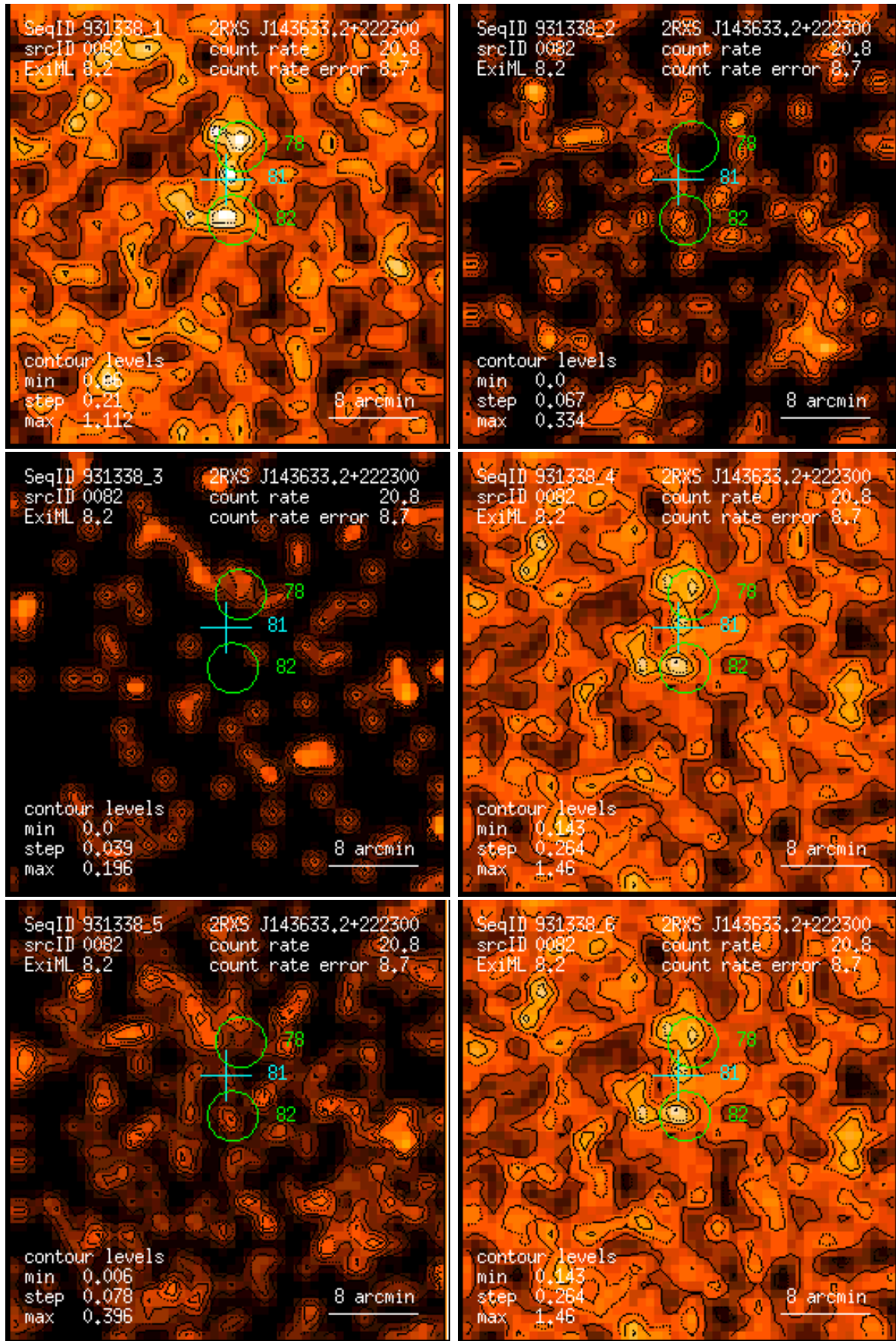
Figure 82: RASS 931338: detection 0082: band rate images, Gaussian filter: (1) PSPC channels 11 – 41, (2) 52 – 90, (3) 91 – 201, (4) 11 – 235, (5) 52 – 201, (6) 11 – 201. Broad band rates in counts/ks. Band rate contour levels in counts/ks/arcmin 2 .
