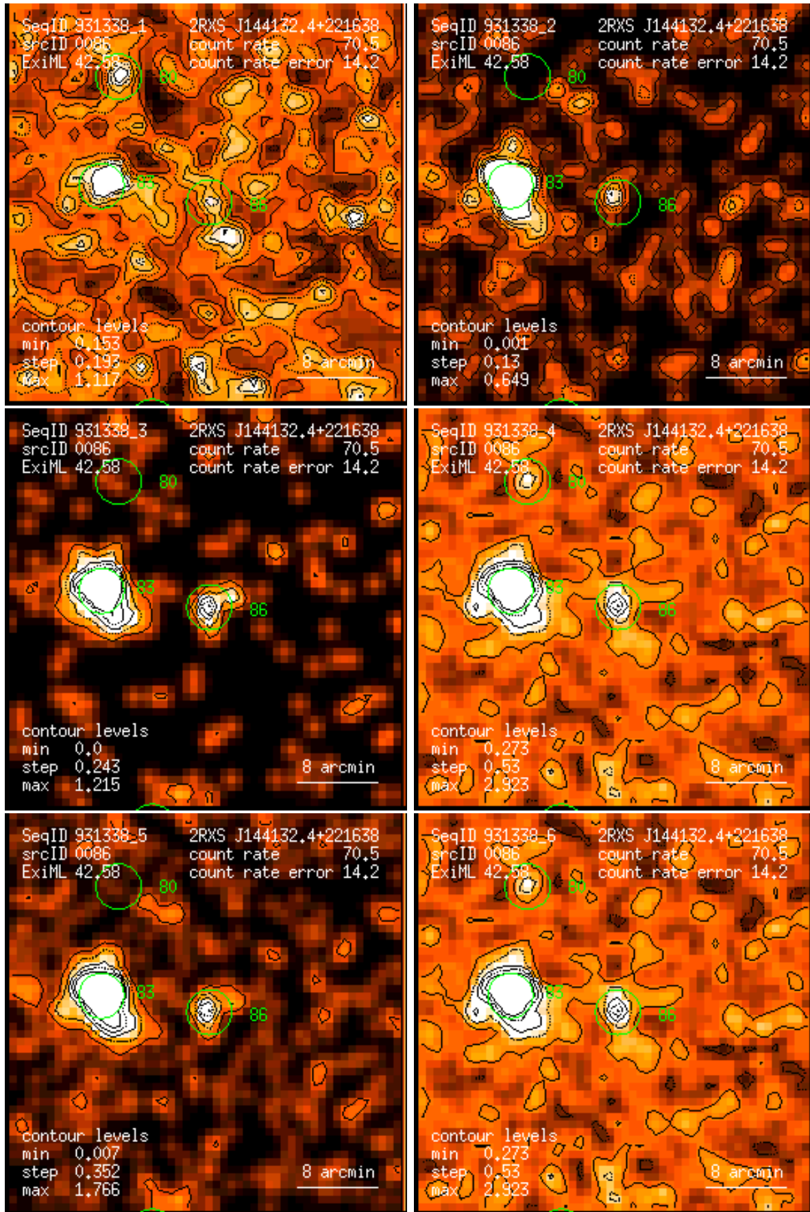
Figure 86: RASS 931338: detection 0086: band rate images, Gaussian filter: (1) PSPC channels 11 – 41, (2) 52 – 90, (3) 91 – 201, (4) 11 – 235, (5) 52 – 201, (6) 11 – 201. Broad band rates in counts/ks. Band rate contour levels in counts/ks/arcmin 2 .
