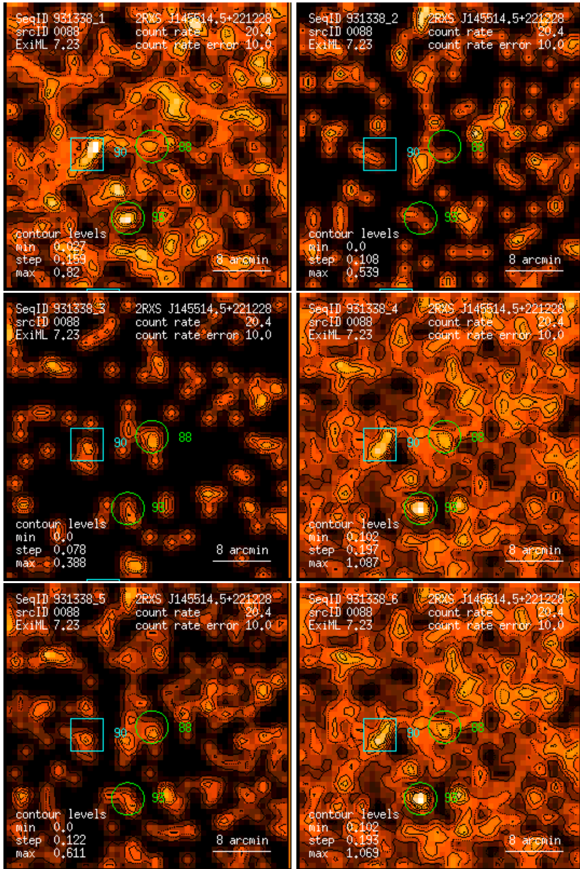
Figure 88: RASS 931338: detection 0088: band rate images, Gaussian filter: (1) PSPC channels 11 – 41, (2) 52 – 90, (3) 91 – 201, (4) 11 – 235, (5) 52 – 201, (6) 11 – 201. Broad band rates in counts/ks. Band rate contour levels in counts/ks/arcmin 2 .
