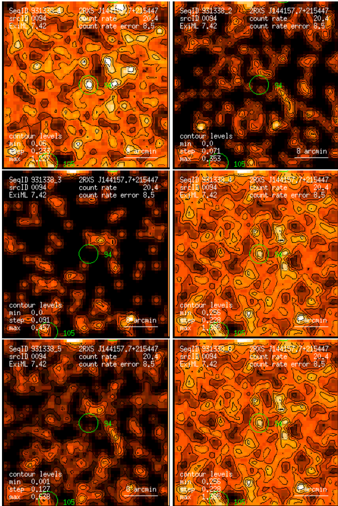
Figure 94: RASS 931338: detection 0094: band rate images, Gaussian filter: (1) PSPC channels 11 – 41, (2) 52 – 90, (3) 91 – 201, (4) 11 – 235, (5) 52 – 201, (6) 11 – 201. Broad band rates in counts/ks. Band rate contour levels in counts/ks/arcmin 2 .
