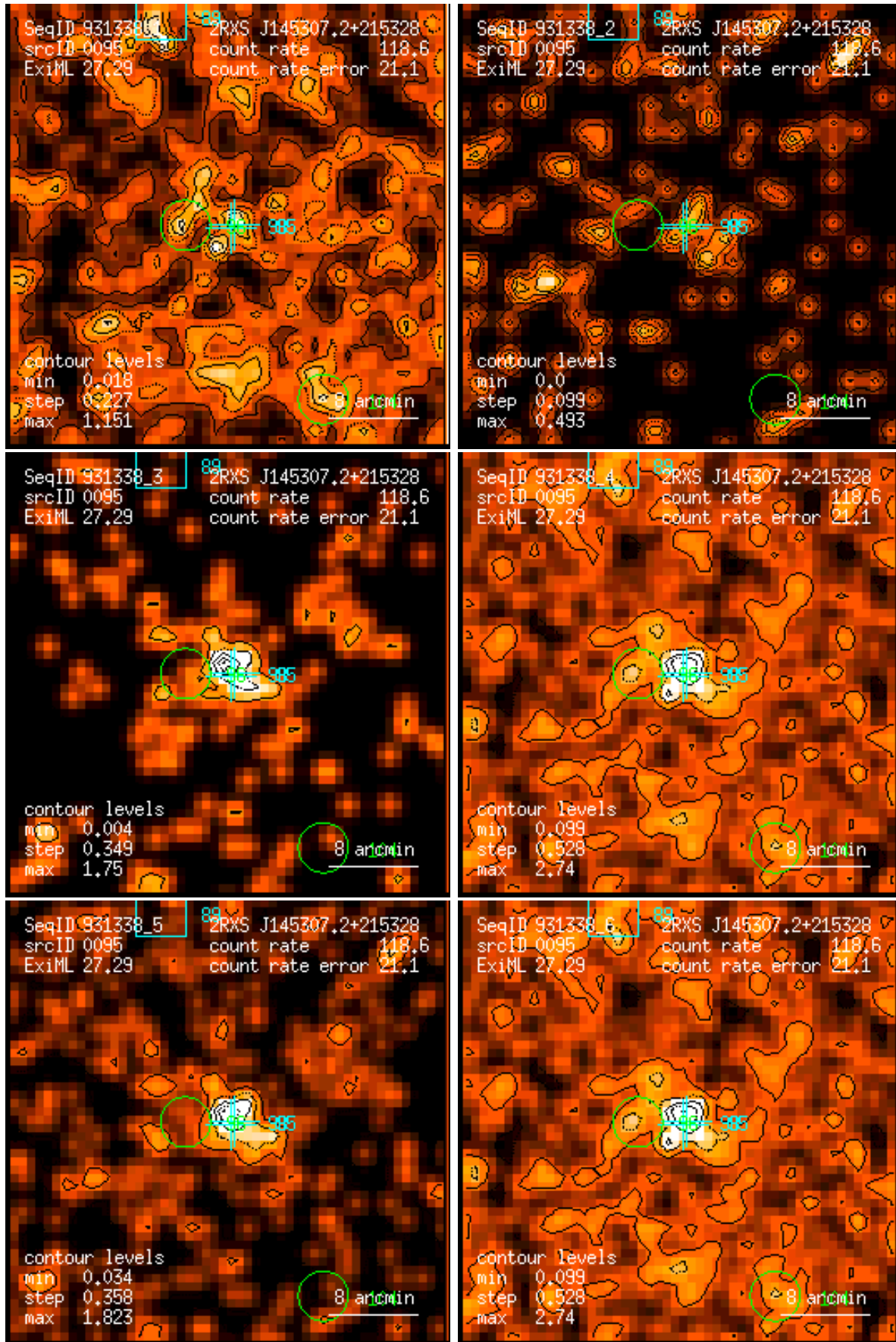
Figure 95: RASS 931338: detection 0095: band rate images, Gaussian filter: (1) PSPC channels 11 – 41, (2) 52 – 90, (3) 91 – 201, (4) 11 – 235, (5) 52 – 201, (6) 11 – 201. Broad band rates in counts/ks. Band rate contour levels in counts/ks/arcmin 2 .
