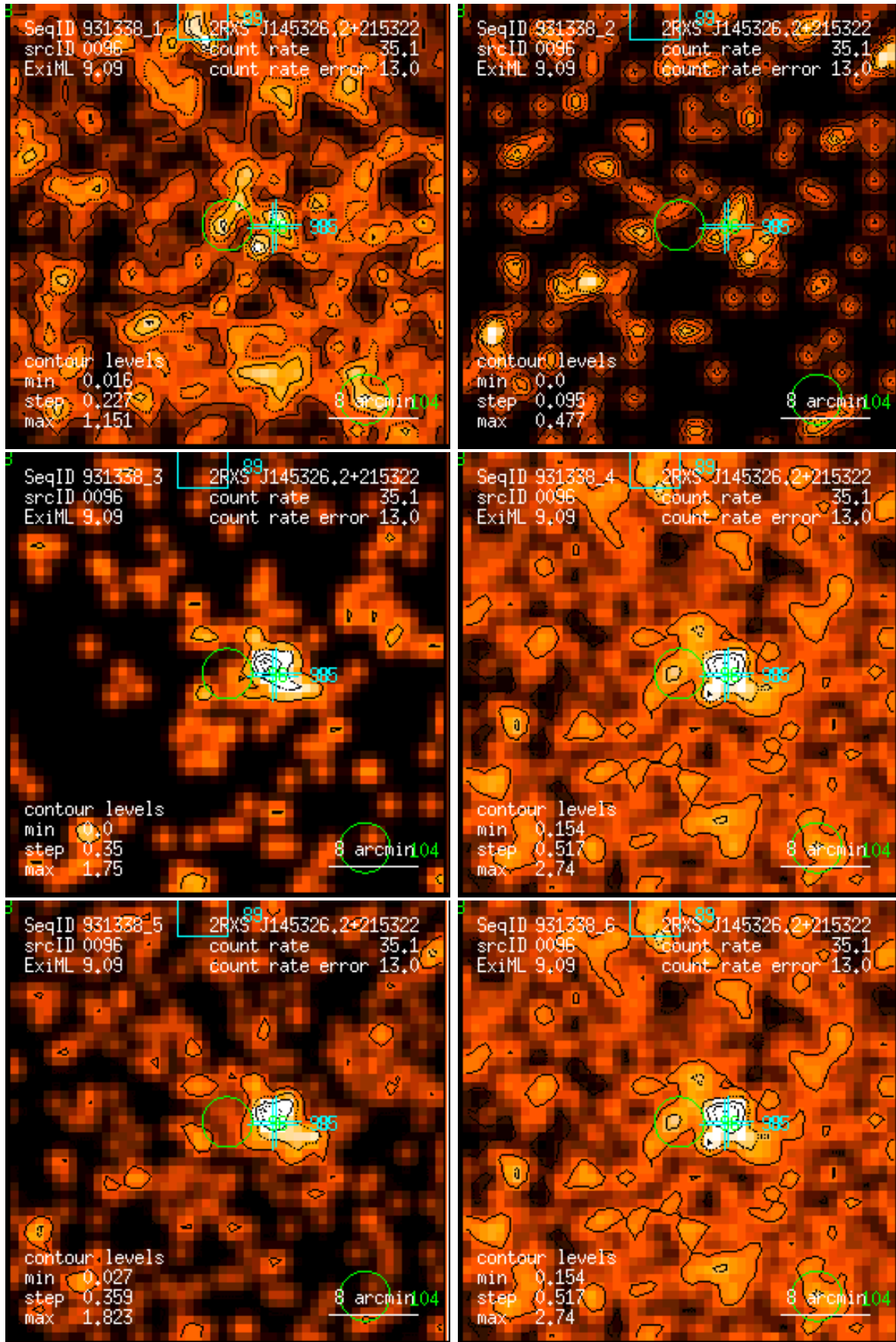
Figure 96: RASS 931338: detection 0096: band rate images, Gaussian filter: (1) PSPC channels 11 – 41, (2) 52 – 90, (3) 91 – 201, (4) 11 – 235, (5) 52 – 201, (6) 11 – 201. Broad band rates in counts/ks. Band rate contour levels in counts/ks/arcmin 2 .
